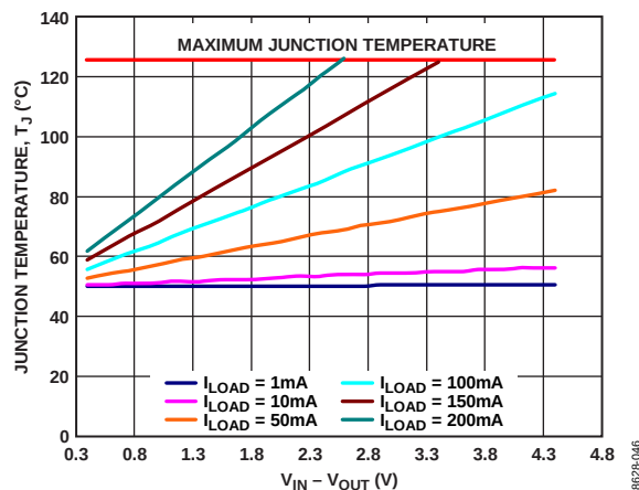
Figure 48. 100 mm² of PCB Copper, TSOT, T_A = 50^\circ\text{C}
