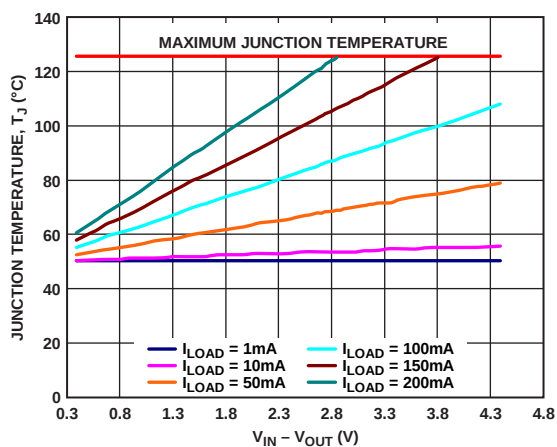
Figure 47. 500 mm² of PCB Copper, TSOT, T_A = 50^\circ\text{C}
