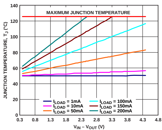
Figure 43. 500 mm² of PCB Copper, WLCSP, T_A = 85^\circ\text{C}
