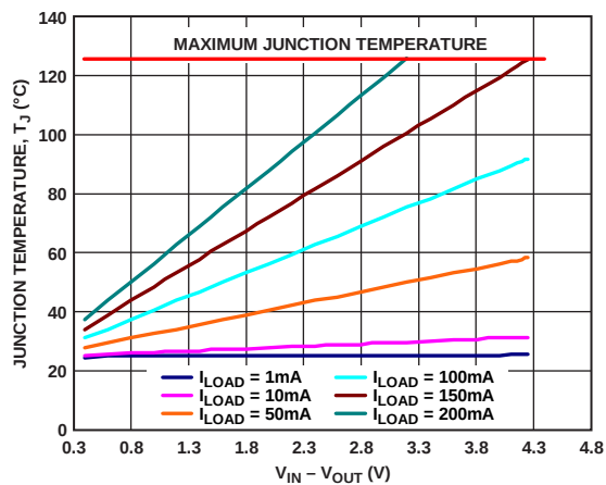
Figure 42. 100 mm² of PCB Copper, WLCSP, T_A = 50^\circ\text{C}
