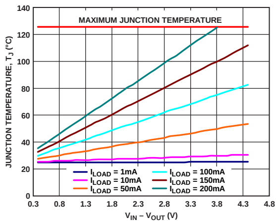
Figure 45. 500 mm² of PCB Copper, TSOT, T_A = 25^\circ\text{C}
