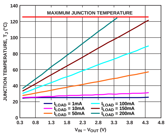
Figure 46. 100 mm² of PCB Copper, TSOT, T_A = 25^\circ\text{C}
