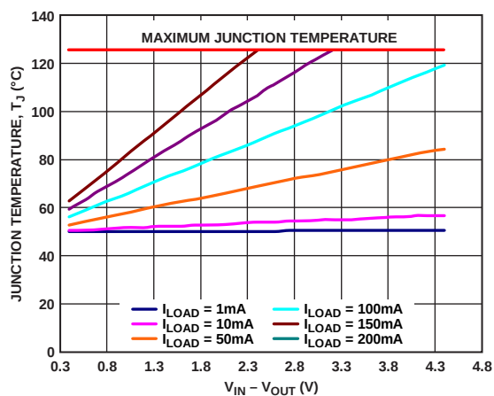
Figure 44. 100 mm² of PCB Copper, WLCSP, T_A = 50^\circ\text{C}
