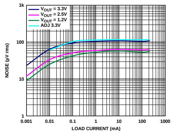
Figure 24. Output Noise vs. Load Current and Output Voltage, V_{IN} = 5V , C_{OUT} = 1\mu F
