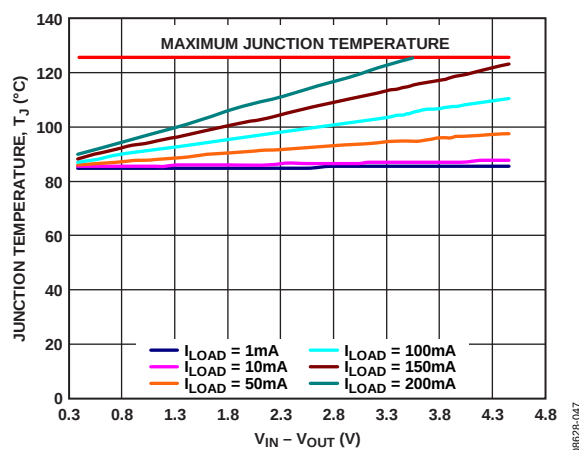
Figure 49. WLCSP, T_A = 85^\circ\text{C}
