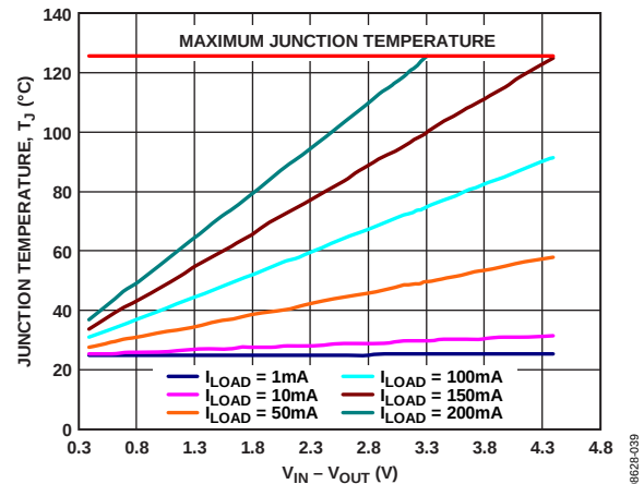
Figure 37. 500 mm 2 of PCB Copper, WLCSP, T_A = 25^\circ\text{C}
