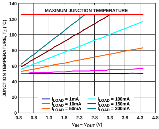
Figure 39. 500 mm² of PCB Copper, WLCSP, T_A = 85^\circ\text{C}
