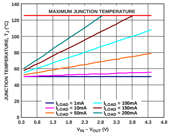
Figure 43. 500 mm² of PCB Copper, TSOT, T_A = 50^\circ\text{C}
