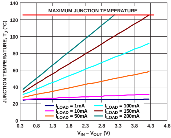
Figure 38. 100 mm² of PCB Copper, WLCSP, T_A = 50^\circ\text{C}
