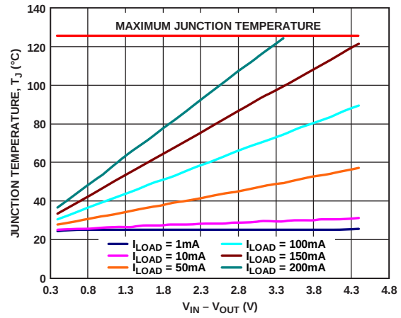
Figure 42. 100 mm² of PCB Copper, TSOT, T_A = 25^\circ\text{C}
