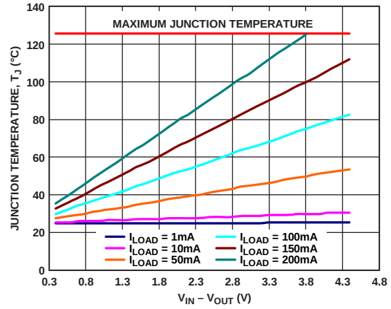
Figure 41. 500 mm² of PCB Copper, TSOT, T_A = 25^\circ\text{C}
