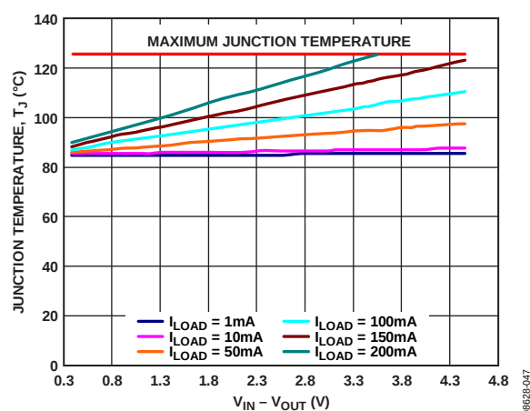
Figure 45. WLCSF, T_A = 85^\circ\text{C}
