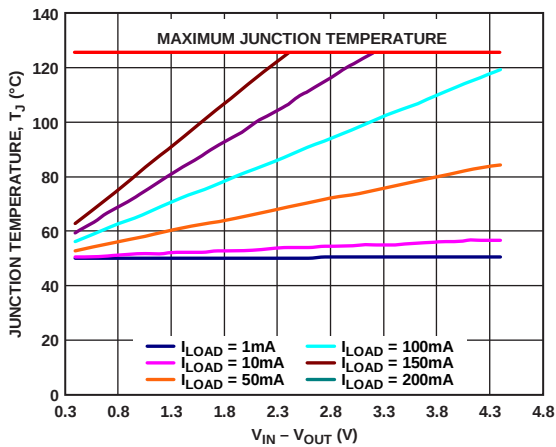
Figure 40. 100 mm² of PCB Copper, WLCSP, T_A = 50^\circ\text{C}
