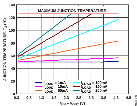
Figure 43. 500 mm² of PCB Copper, WLCSP, T_A = 85^\circ\text{C}
