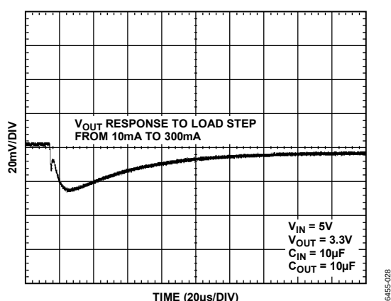
Figure 32. Output Transient Response, C_{OUT} = 10 \mu\text{F}
