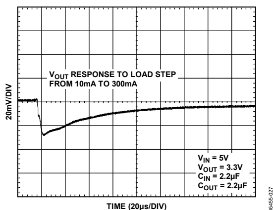
Figure 31. Output Transient Response, C_{OUT} = 2.2 \mu\text{F}
