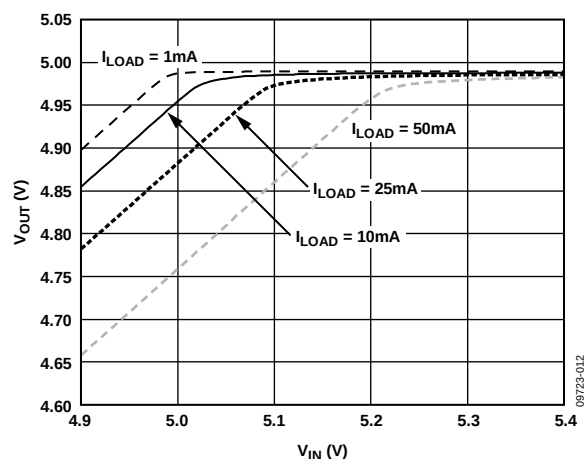
Figure 12. Output Voltage vs. Input Voltage (in Dropout)
