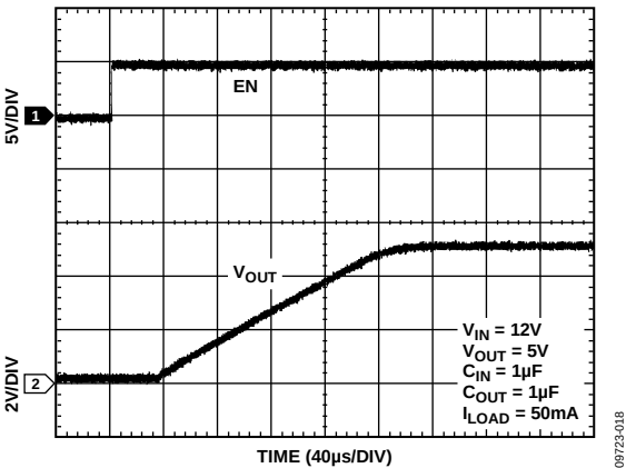
Figure 18. Start-Up Time
