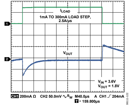
Figure 20. Load Transient Response, C_{IN} and C_{OUT} = 4.7\text{ }\mu\text{F}
