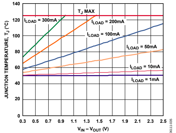
Figure 35. 0 mm² of PCB Copper, T_A = 50^\circ\text{C}
