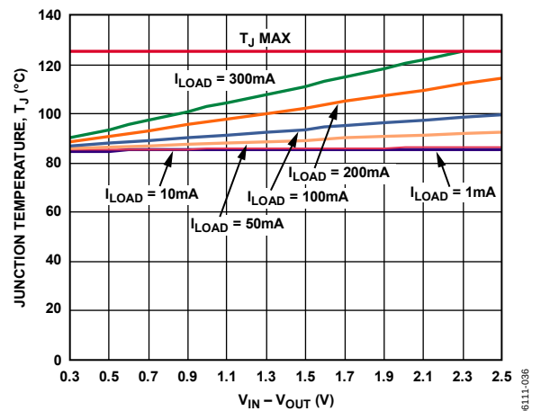
Figure 36. T_A = 85^\circ\text{C}
