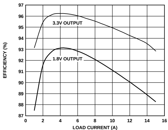
Figure 2. Efficiency vs. Load Current, 5 V Input
