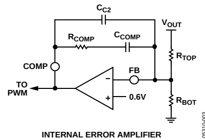
Figure 15. Compensation Using the ESR Zero
