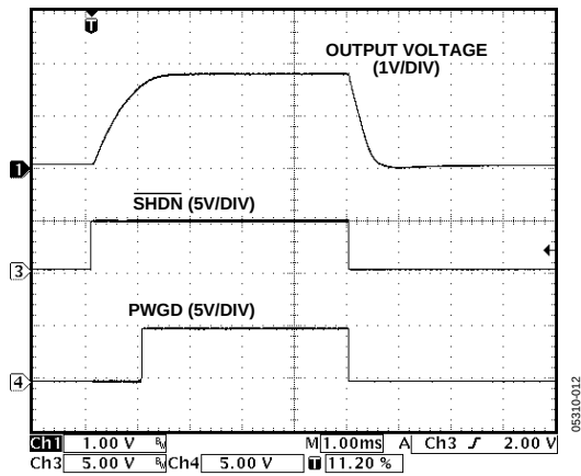
Figure 12. Power-On Response
