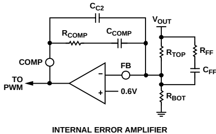
Figure 16. Compensation Using Feed Forward
