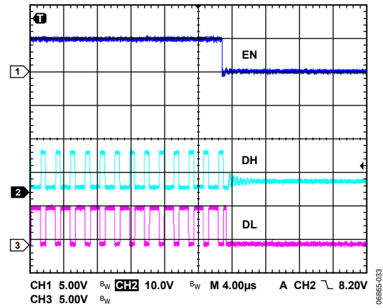
Figure 33. EN, Shutdown
