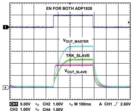
Figure 51. Ratiometric Tracking of Figure 47 with R_{TRKT} = 5k\Omega
