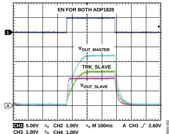
Figure 50. Ratiometric Tracking of Figure 46 with R_{TRKT} = 5 \text{ k}\Omega
