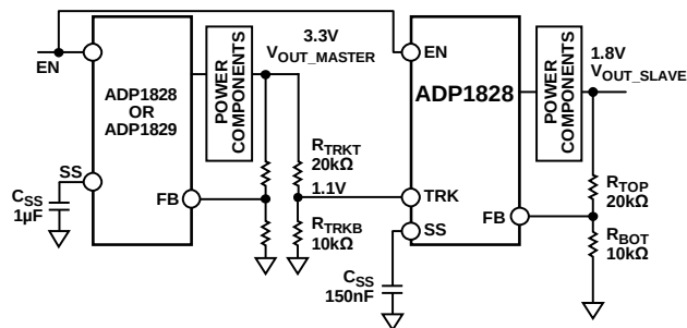
Figure 42. Example of a Coincident Tracking Circuit
