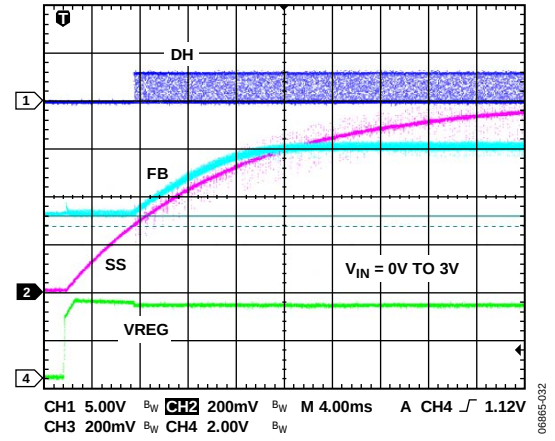
Figure 31. Start into Precharged Output
