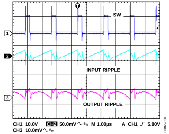
Figure 20. Input and Output Ripple of Figure 54, 4 A Load
