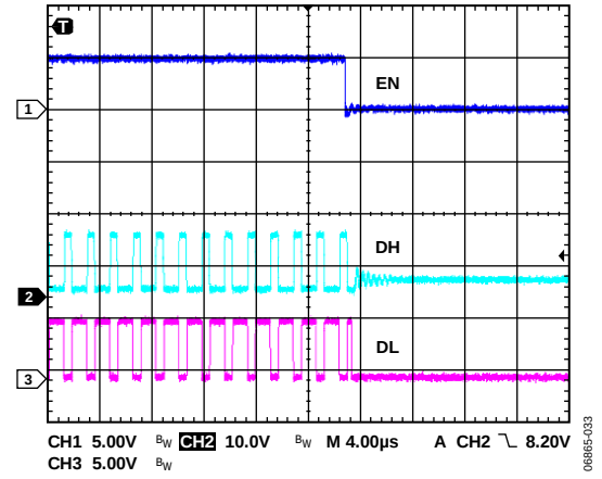
Figure 32. EN, Shutdown
