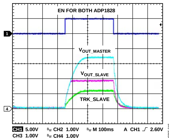
Figure 44. Coincident Tracking of Figure 42
