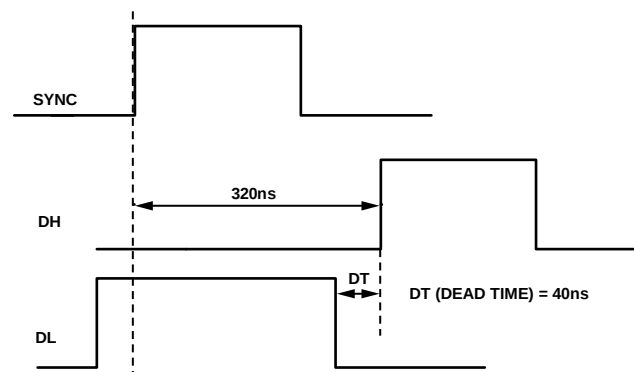
Figure 34. Synchronization
