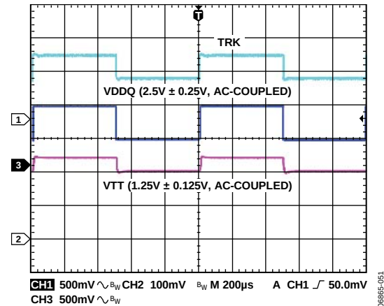
Figure 49. DDR Termination; Output Waveforms of Figure 48
