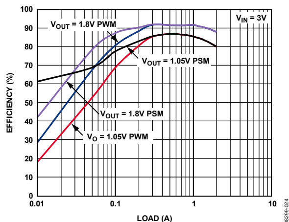
Figure 6. Efficiency Plot of Figure 44, 2 A Output
