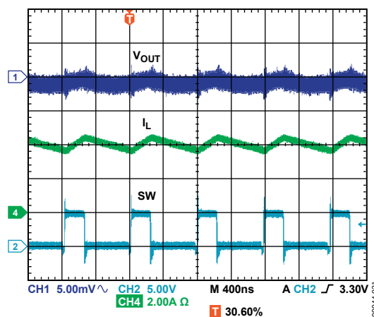
Figure 31. Steady Waveform, V_{IN} = 5\text{ V} , V_{OUT} = 1.2\text{ V} , f_s = 1.2\text{ MHz}
