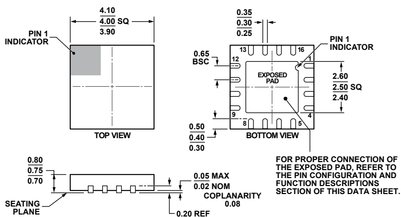
Figure 48. 16-Lead Lead Frame Chip Scale Package [LFCSP_WQ] 4 mm × 4 mm Body, Very Very Thin Quad (CP-16-26)
