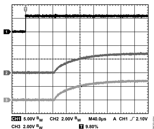
Figure 34. Typical Start-Up Time
