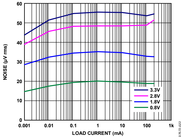
Figure 22. Output Noise vs. Load Current and Output Voltage, V_{IN} = 5V
