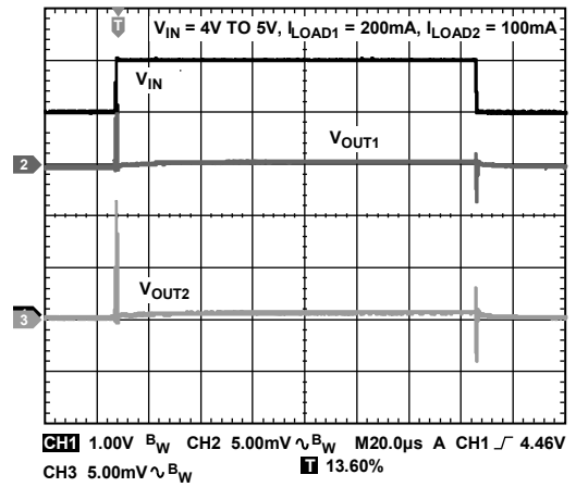
Figure 25. Line Transient Response, V_{IN} = 4V to 5V , I_{LOAD1} = 200mA , I_{LOAD2} = 100mA CH1 = V_{IN} , CH2 = V_{OUT1} , CH3 = V_{OUT2}
