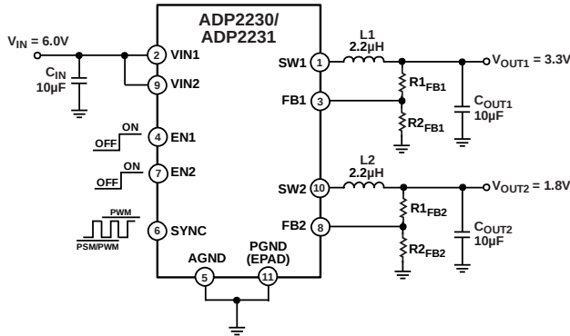
Figure 33. Typical Application Circuit Adjustable Output Voltage
