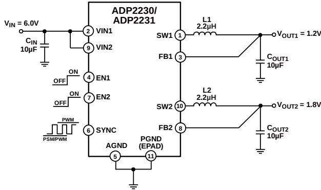
Figure 32. Typical Application Circuit Fixed Output Voltage
