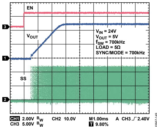
Figure 48. Startup with Precision Enable, V_{IN} = 24V , V_{OUT} = 5V , f_{SW} = 700kHz , Load = 5Ω, SYNC/MODE = 700kHz
