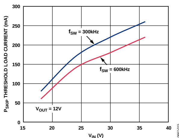
Figure 21. Pulse Skip Threshold Load Current, V_{OUT} = 12V
