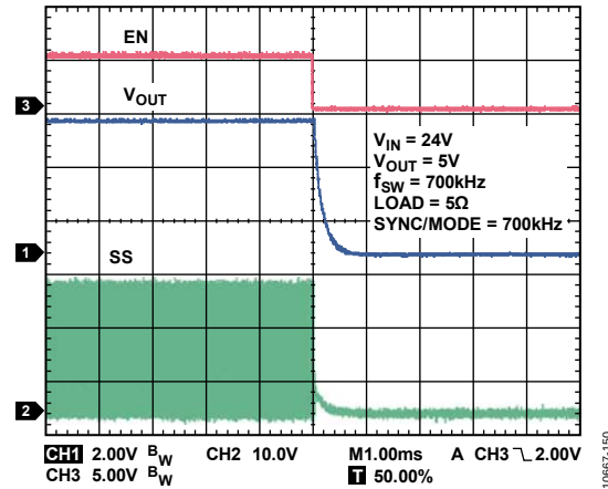
Figure 49. Shutdown with Precision Enable, V_{IN} = 24V , V_{OUT} = 5V , f_{SW} = 700kHz , Load = 5Ω, SYNC/MODE = 700kHz
