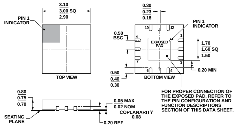
Figure 72. 12-Lead Lead Frame Chip Scale Package [LFCSP_WQ] 3 mm × 3 mm Body, Very Very Thin Quad (CP-12-6) Dimensions shown in millimeters
