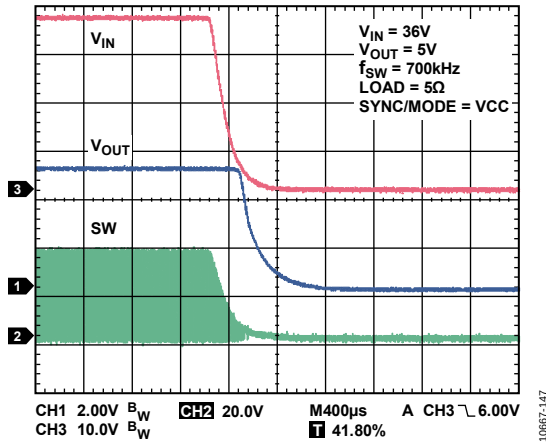
Figure 46. Shutdown with V_{IN} , PWM Mode, V_{IN} = 36V , V_{OUT} = 5V , f_{SW} = 700kHz , Load = 5Ω, SYNC/MODE = VCC
