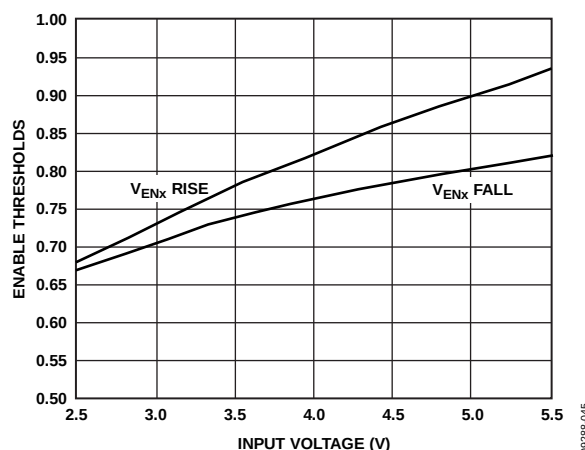
Figure 48. Typical ENx Pins Thresholds vs. Input Voltage
