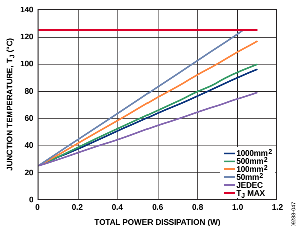
Figure 50. Junction Temperature vs. Total Power Dissipation, T_A = 25^\circ\text{C}
