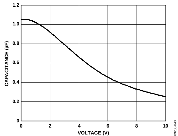
Figure 46. Capacitance vs. Voltage Bias Characteristic
