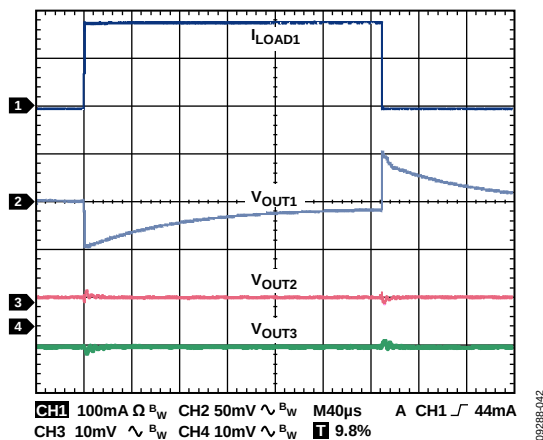
Figure 45. Output Transient Response, I_{LOAD1} = 1 \text{ mA} to 200 \text{ mA} , I_{LOAD2} = 1 \text{ mA} , I_{LOAD3} = 1 \text{ mA} , CH1 = I_{LOAD1} , CH2 = V_{OUT1} , CH3 = V_{OUT2} , CH4 = V_{OUT3}
