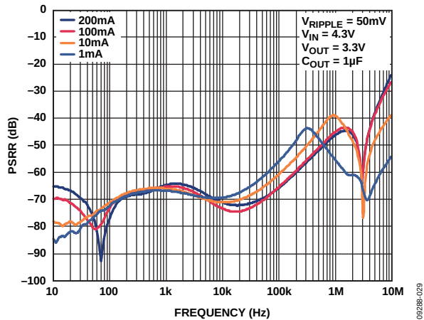
Figure 31. Power Supply Rejection Ratio vs. Frequency, 3.3\text{ V}
