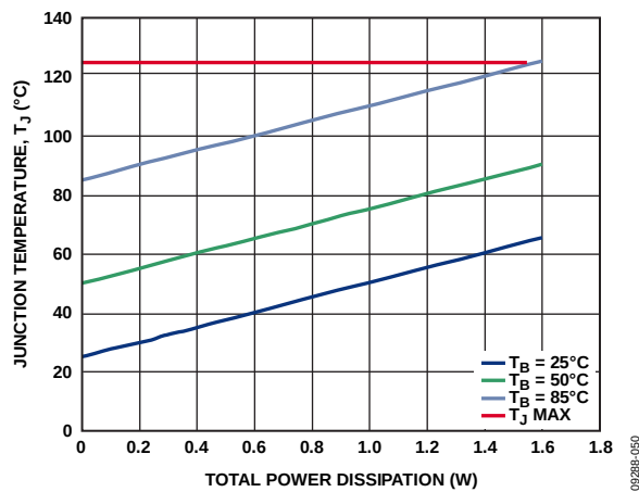
Figure 53. Junction Temperature vs. Total Power Dissipation and Board Temperature
