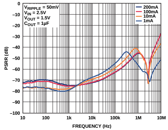
Figure 32. Power Supply Rejection Ratio vs. Frequency, 1.5\text{ V}
