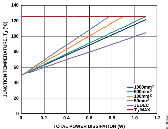
Figure 51. Junction Temperature vs. Total Power Dissipation, T_A = 50^\circ\text{C}
