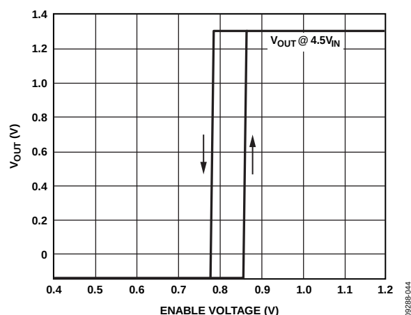
Figure 47. Typical ENx Pin Operation
