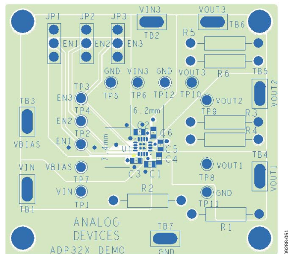
Figure 54. Example of PCB Layout, Top Side
