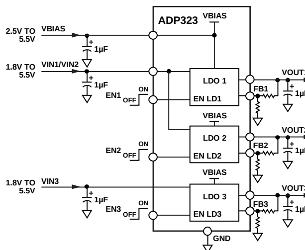
Figure 2. Typical Application Circuit for ADP323
