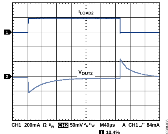
Figure 38. Load Transient Response, I_{LOAD2} = 1mA to 200mA , C_{OUT2} = 1\mu F , CH1 = I_{LOAD2} , CH2 = V_{OUT2}
