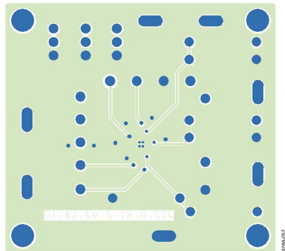
Figure 55. Example of PCB Layout, Bottom Side
