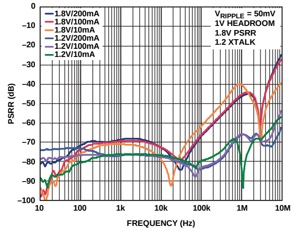
Figure 33. Power Supply Rejection Ratio vs. Frequency, Channel-to-Channel Crosstalk
