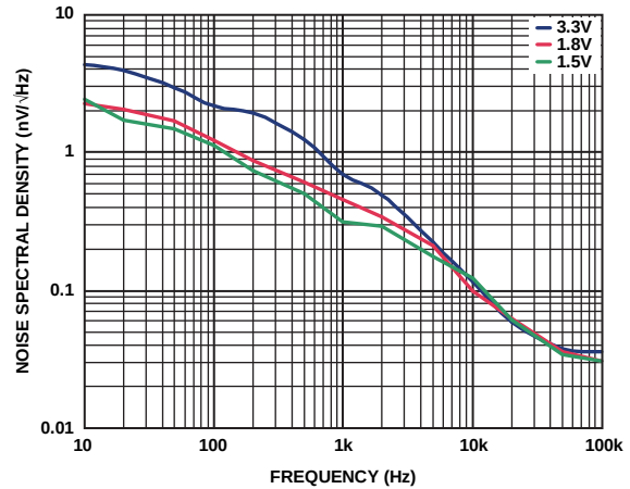
Figure 34. Output Noise Spectral Density vs. Frequency, V_{IN} = 5\text{ V} , I_{LOAD} = 10\text{ mA}
