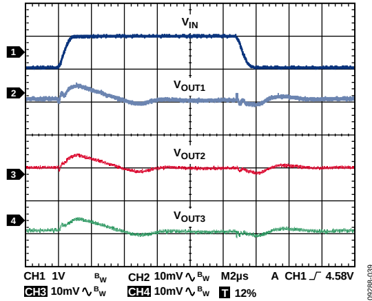
Figure 41. Line Transient Response, V_{IN} = 4V to 5V , I_{LOAD1} = I_{LOAD2} = I_{LOAD3} = 1mA , CH1 = V_{IN} , CH2 = V_{OUT1} , CH3 = V_{OUT2} , CH4 = V_{OUT3}
