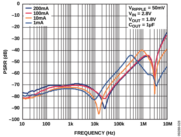
Figure 30. Power Supply Rejection Ratio vs. Frequency, 1.8\text{ V}
