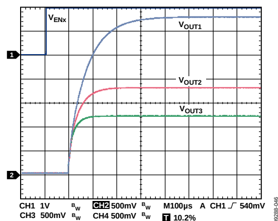
Figure 49. Typical Start-Up Time, I_{LOAD1} = I_{LOAD2} = I_{LOAD3} = 100\text{ mA} , CH1 = V_{ENx} (the Enable Voltage), CH2 = V_{OUT1} , CH3 = V_{OUT2} , CH4 = V_{OUT3}
