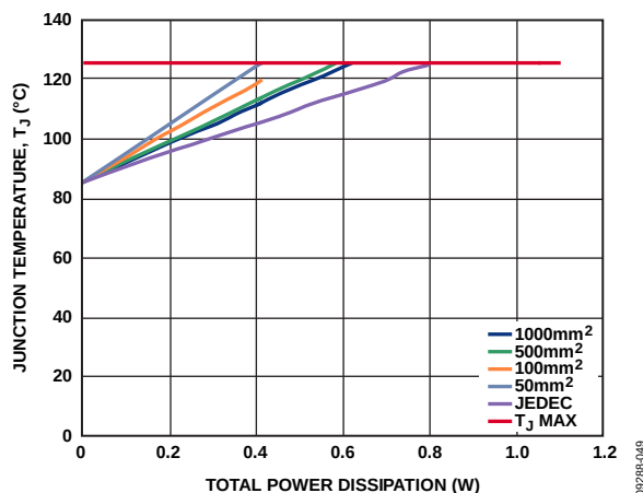
Figure 52. Junction Temperature vs. Total Power Dissipation, T_A = 85^\circ\text{C}
