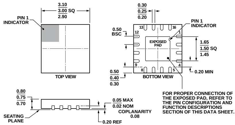
Figure 56. 16-Lead Lead Frame Chip Scale Package [LFCSP_WQ] 3 mm × 3 mm Body, Very, Very Thin Quad (CP-16-27) Dimensions shown in millimeters
