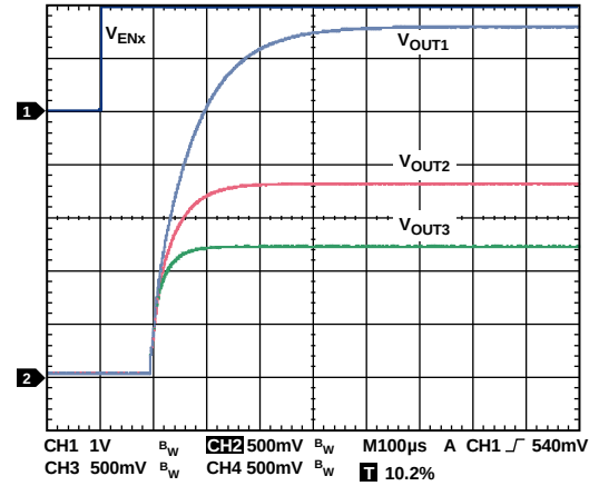
Figure 42. Turn-On Response, I_{LOAD1} = I_{LOAD2} = I_{LOAD3} = 100mA , CH1 = V_{ENx} (the Enable Voltage), CH2 = V_{OUT1} , CH3 = V_{OUT2} , CH4 = V_{OUT3}
