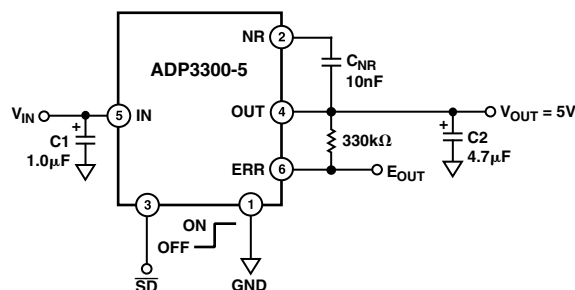
Figure 3. Noise Reduction Circuit
