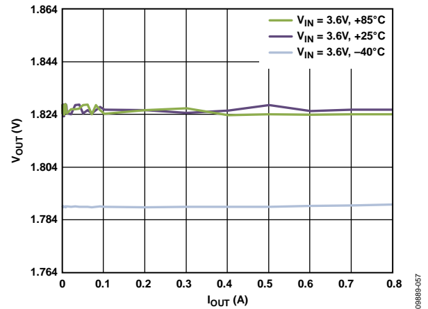
Figure 7. BUCK2 Load Regulation Across Temperature, V_{OUT2} = 1.8\text{ V} , Auto Mode
