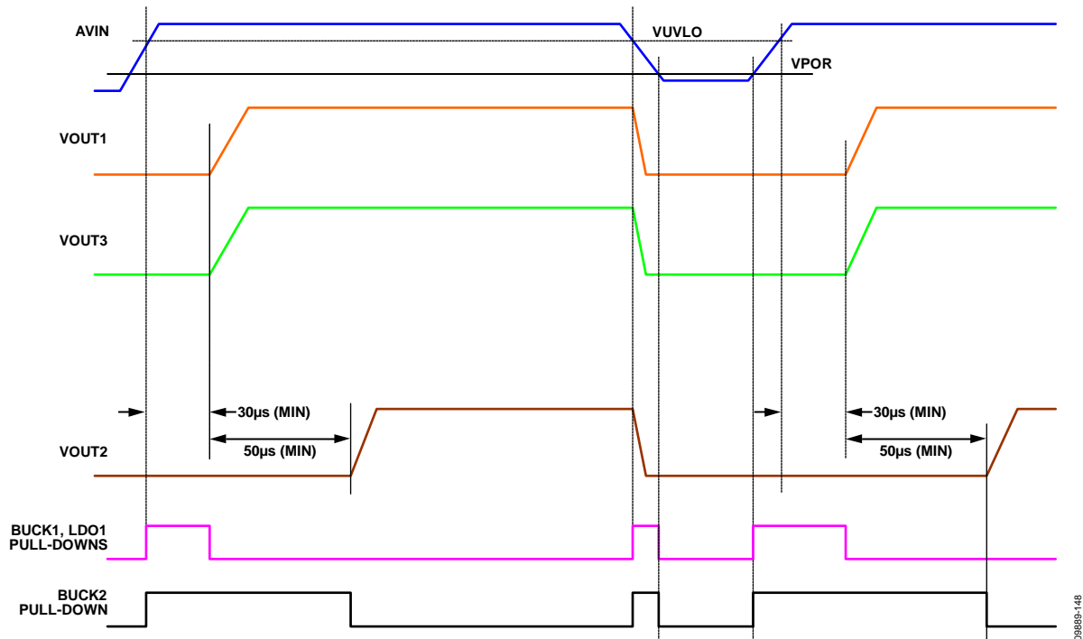
Figure 46. Regulator Sequencing on ADP5023 (EN1 = EN2 = EN3 = V_{AVIN} )
