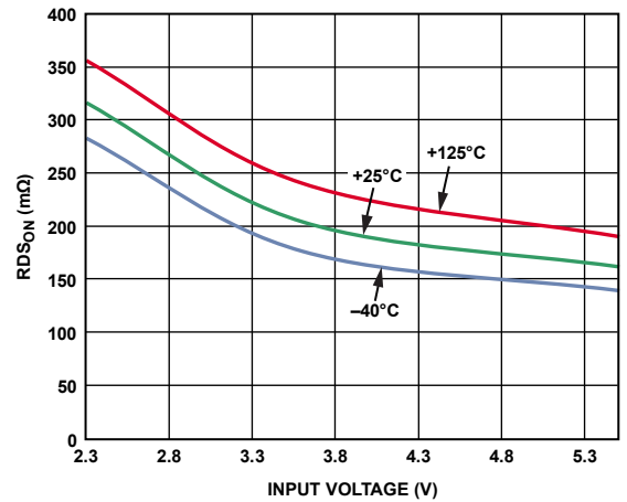
Figure 32. NMOS R_{DS(on)} vs. V_{INx}
