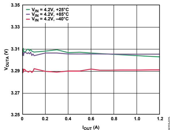
Figure 6. BUCK1 Load Regulation Across Temperature, V_{OUT1} = 3.3\text{ V} , Auto Mode
