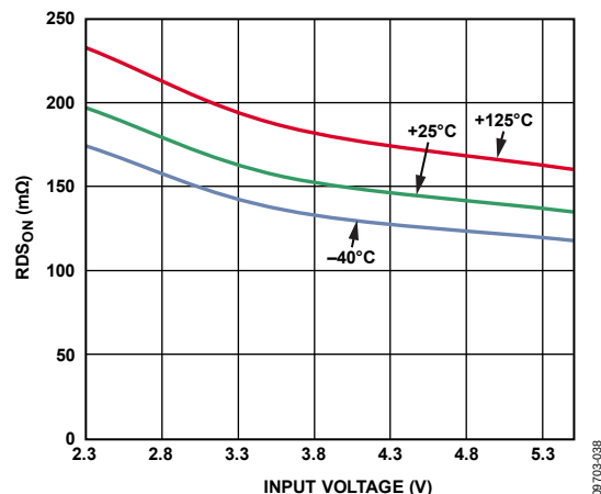
Figure 33. PMOS R_{DS(on)} vs. V_{IN}
