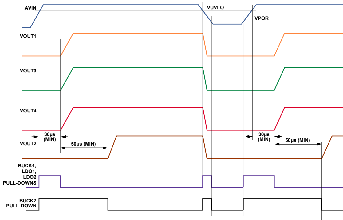
Figure 46. Regulator Sequencing on the ADP5034 (EN1 = EN2 = EN3 = EN4 = V AVIN )
