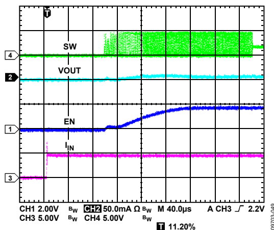
Figure 4. BUCK1 Startup, V_{OUT1} = 3.3\text{ V} , I_{OUT1} = 10\text{ mA}
