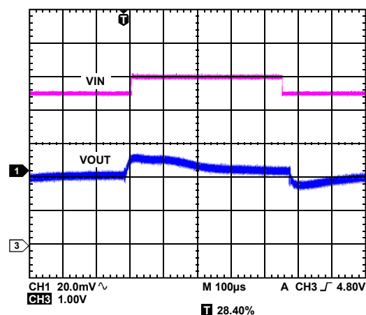
Figure 38. LDO Response to Line Transient, Input Voltage from 4.5 V to 5.5 V, V_{OUT3} = 2.8\text{ V}
