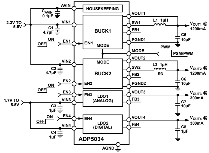
Figure 52. ADP5034 Fixed Output Voltages with Enable Pins
