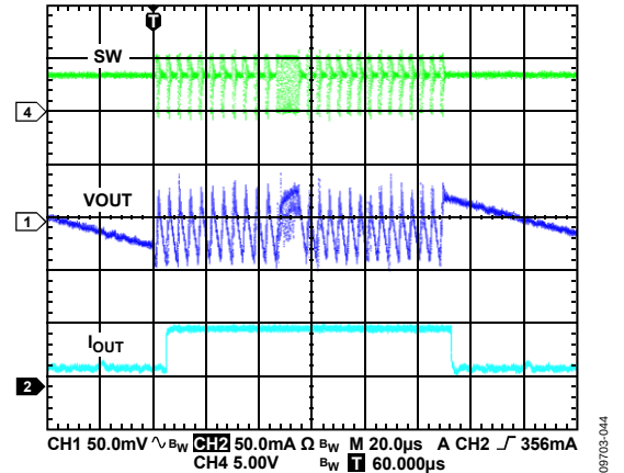
Figure 25. BUCK1 Response to Load Transient, I_{OUT1} from 1\text{ mA} to 50\text{ mA} , V_{OUT1} = 3.3\text{ V} , Auto Mode
