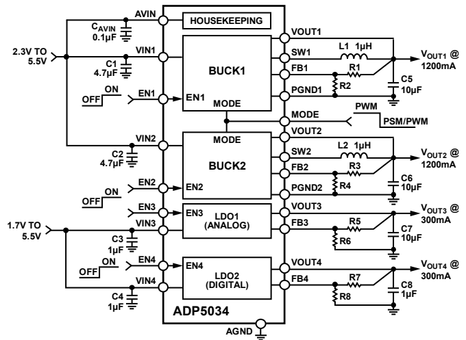
Figure 53. ADP5034 Adjustable Output Voltages with Enable Pins
