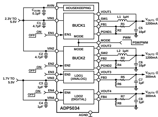
Figure 51. Processor System Power Management with PSM/PWM Control
