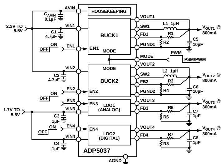
Figure 53. ADP5037 Adjustable Output Voltages with Enable Pins
