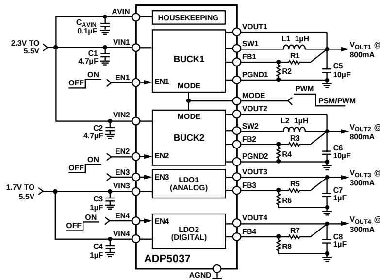
Figure 50. Processor System Power Management with PSM/PWM Control
