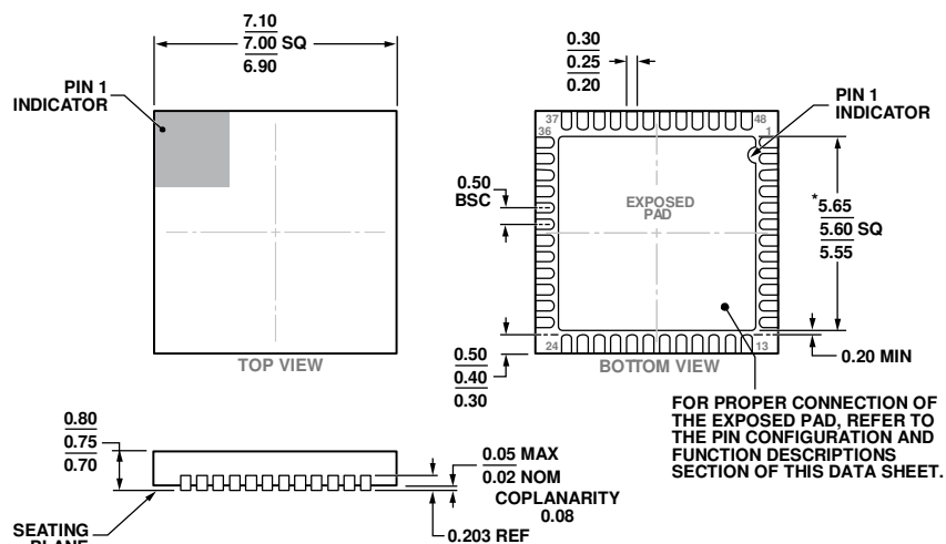
Figure 55. 48-Lead Lead Frame Chip Scale Package [LFCSP_WQ] 7 mm × 7 mm Body, Very Very Thin Quad (CP-48-13)
