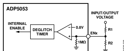
Figure 33. Precision Enable Diagram for One Channel
