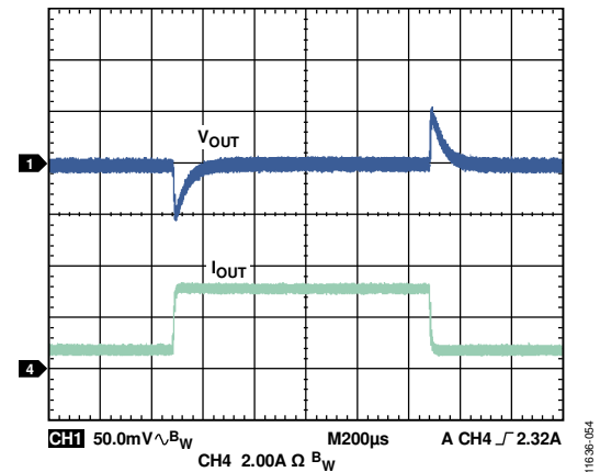
Figure 49. 0.8 A to 3.2 A Load Transient for 1.2 V Output
