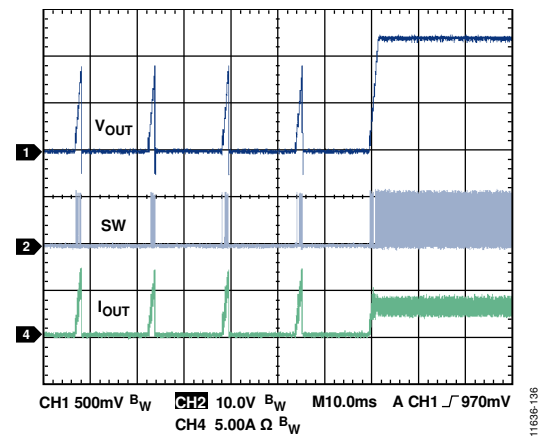
Figure 31. Short-Circuit Protection Recovery, V_{IN} = 12\text{ V} , V_{OUT} = 1.2\text{ V} , f_{SW} = 600\text{ kHz} , L = 1\text{ μH} , C_{OUT} = 47\text{ μF} \times 2
