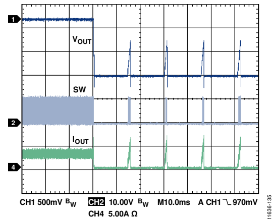
Figure 30. Short-Circuit Protection Entry, V_{IN} = 12\text{ V} , V_{OUT} = 1.2\text{ V} , f_{SW} = 600\text{ kHz} , L = 1\text{ μH} , C_{OUT} = 47\text{ μF} \times 2
