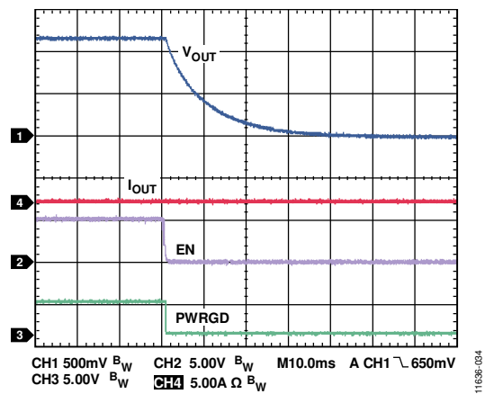
Figure 29. Channel 1/Channel 2 Shutdown with Active Output Discharge, V_{IN} = 12\text{ V} , V_{OUT} = 1.2\text{ V} , f_{SW} = 600\text{ kHz} , L = 1\text{ μH} , C_{OUT} = 47\text{ μF} \times 2
