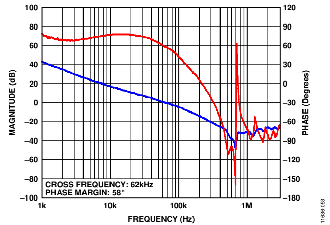
Figure 48. Bode Plot for 1.2 V Output
