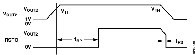
Figure 43. Reset Timing Diagram
