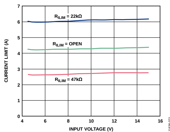
Figure 21. Channel 1/Channel 2 Current Limit vs. Input Voltage
