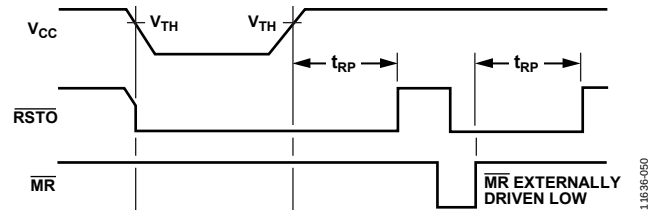
Figure 45. \overline{MR} Timing Diagram in Processor Reset Mode
