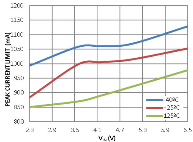
Figure 21. Peak Current Limit vs. V_{IN}
