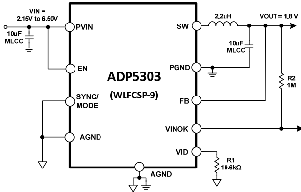
Figure 40. Typical Application Circuit
