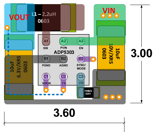
Figure 41. Typical PCB Layout for the ADP5303
