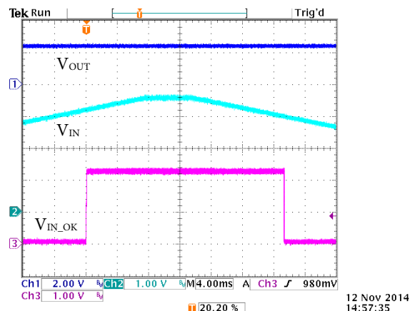
Figure 33. VINOK Function at VINOK Threshold = 3.0 V
