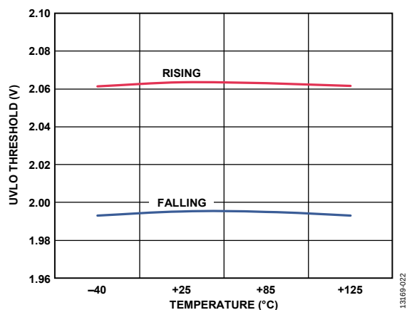
Figure 22. UVLO Threshold, Rising and Falling, vs. Temperature
