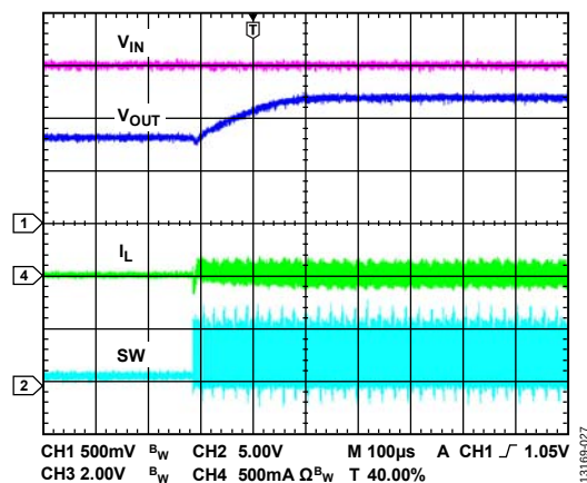
Figure 27. Soft Start with Precharge Function
