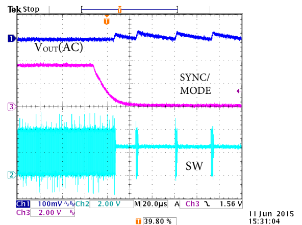
Figure 39. PWM Mode to Hysteresis Mode with 10 mA Load Current
