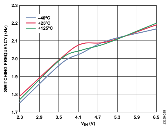
Figure 25. Switching Frequency vs. V_{IN}
