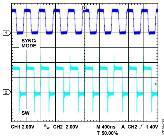
Figure 35. Synchronized to 2.5 MHz
