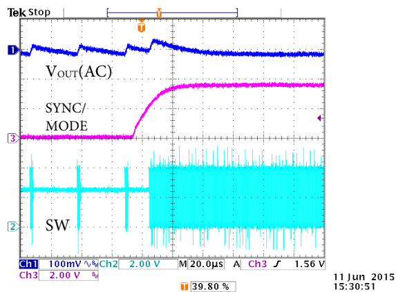
Figure 36. Hysteresis Mode to PWM Mode with 10 mA Load Current
