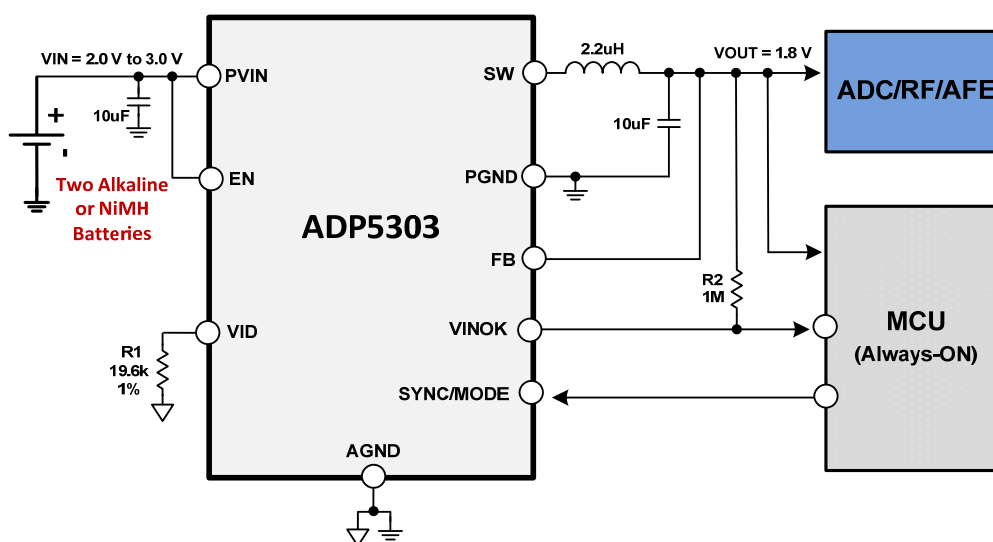
Figure 43. Typical Application Circuit with 2 Alkaline or NiMH Batteries
