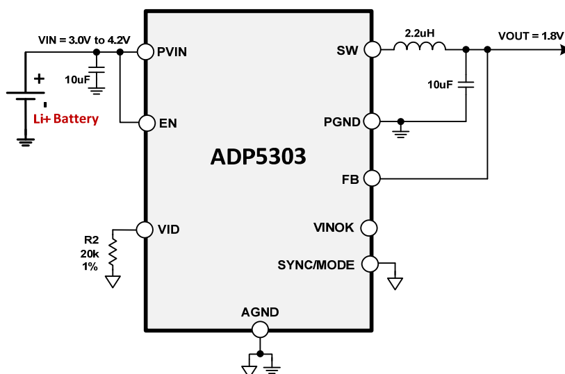
Figure 42. Typical Application Circuit with Li-ion Battery
