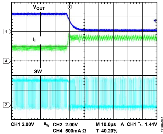
Figure 34. Output Short
