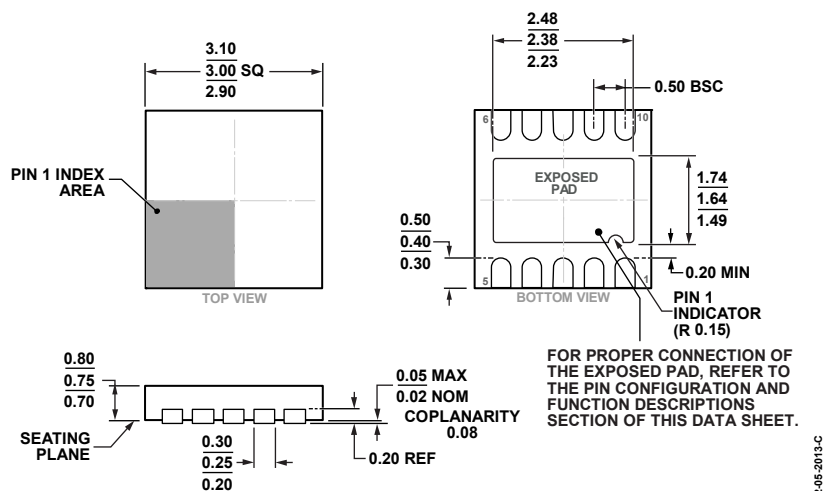
Figure 30. 10-Lead Lead Frame Chip Scale Package [LFCSP_WD] 3 mm × 3 mm Body, Very Very Thin, Dual Lead (CP-10-9)
