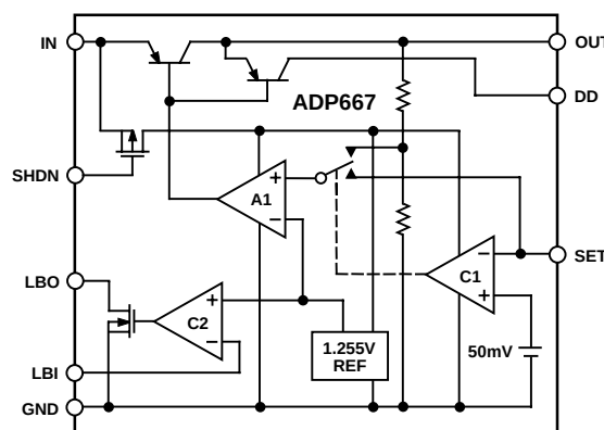
Figure 1. ADP667 Functional Block Diagram
