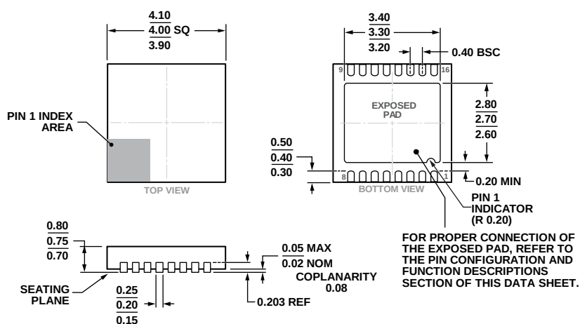
Figure 37. 16-Lead Lead Frame Chip Scale Package [LFCSP_WD] 4 mm × 4 mm Body, Very Very Thin Dual (CP-16-29) Dimensions shown in millimeters
