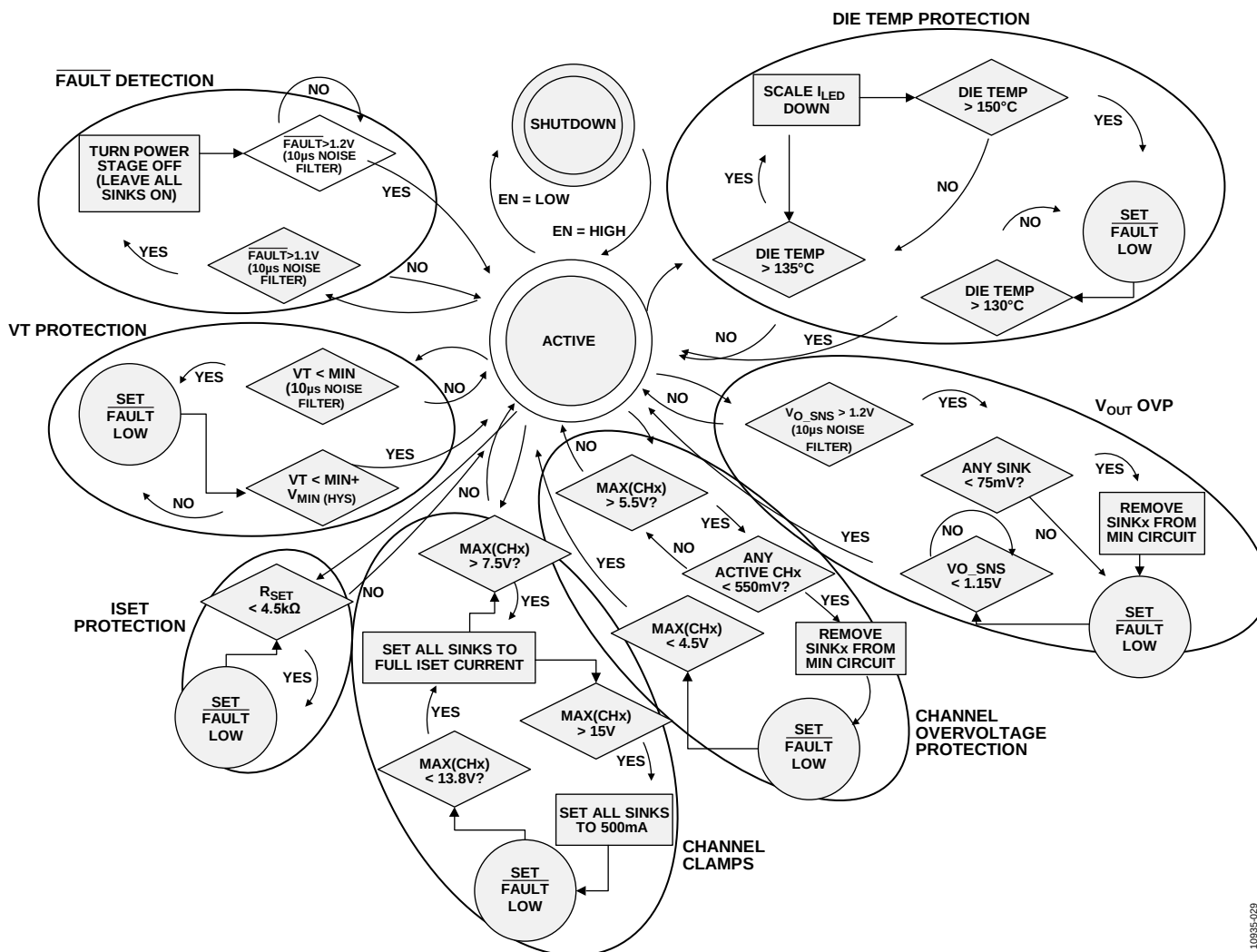
Figure 27. Fault Flowchart
