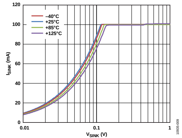
Figure 9. Typical Sink Current vs. Sink Voltage, R_{SET} = 25.5\text{ k}\Omega
