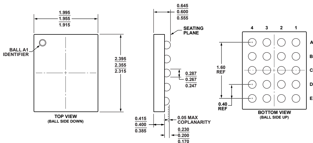
Figure 47. 20-Ball Wafer Level Chip Scale Package [WLCSP] (CB-20-6)
