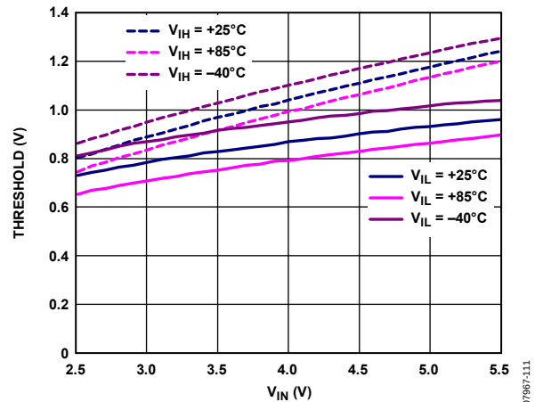
Figure 16. Typical P_C Thresholds, V_{IH} and V_{IL}
