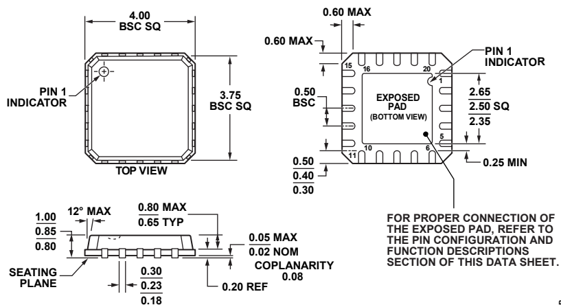
Figure 48. 20-Lead Lead Frame Chip Scale Package [LFCSP_VQ] 4 mm × 4 mm Body, Very Thin Quad (CP-20-4)
