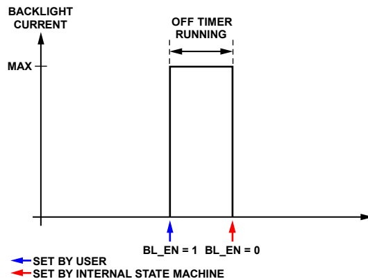
Figure 35. Off Timer
