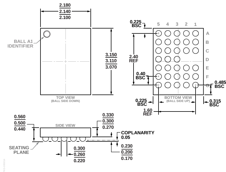
Figure 59. 33-Ball Wafer Level Chip Scale Package [WLCSP] (CB-33-1)
