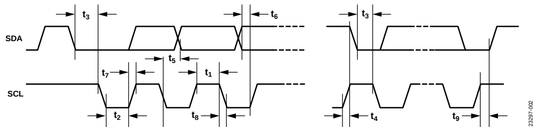
Figure 2. I 2 C Timing Diagram for the ADPD4101
