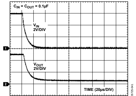
Figure 37. ADR125 Turn-Off Response
