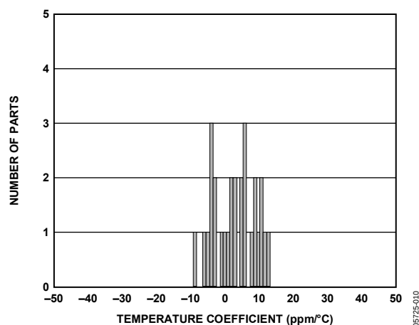
Figure 6. ADR125 Temperature Coefficient
