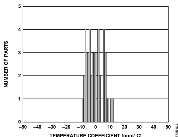
Figure 7. ADR121 Temperature Coefficient
