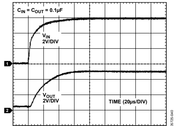
Figure 36. ADR125 Turn-On Response
