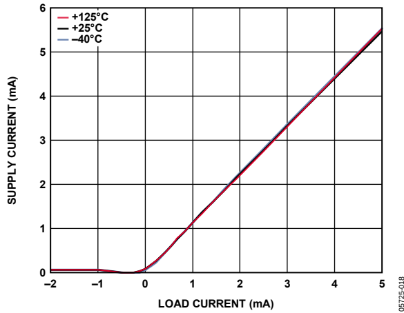
Figure 14. ADR127 Supply Current vs. Load Current
