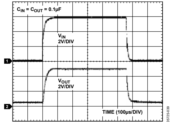
Figure 35. ADR125 Turn-On Response
