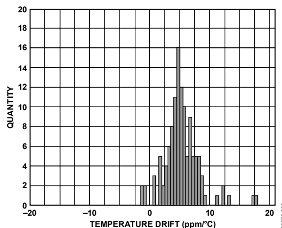
Figure 2. Reverse Voltage Temperature Drift Distribution
