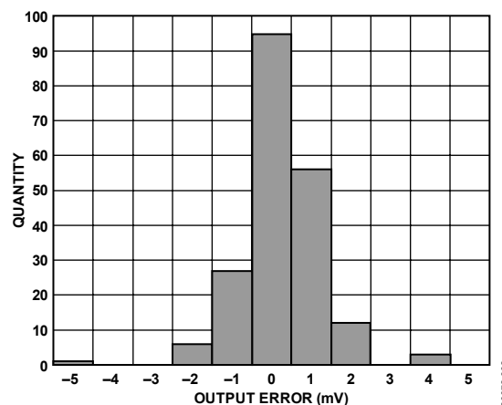
Figure 3. Reverse Voltage Error Distribution
