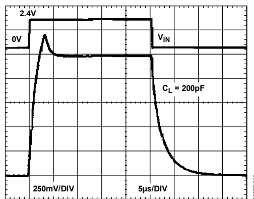
Figure 18. Turn-On Response Time
