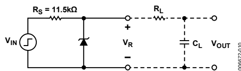
Figure 19. Turn-On, Settling, and Transient Test Circuit
