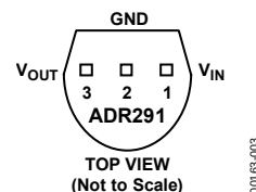
Figure 3. 3-Lead TO-92 (T-3)
