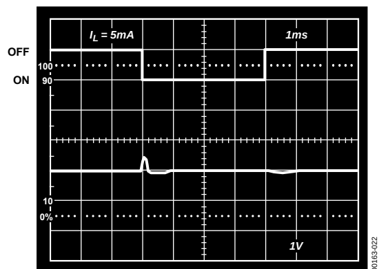
Figure 25. ADR291 Load Transient
