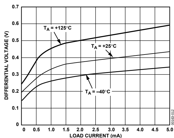
Figure 15. ADR292 Minimum Input-Output Voltage Differential vs. Load Current
