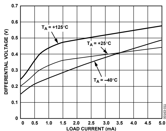
Figure 14. ADR291 Minimum Input-Output Voltage Differential vs. Load Current
