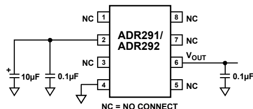
Figure 32. Basic Voltage Reference Configuration
