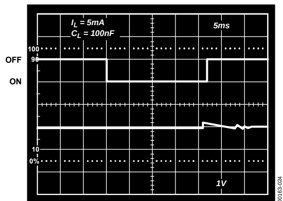
Figure 27. ADR291 Load Transient
