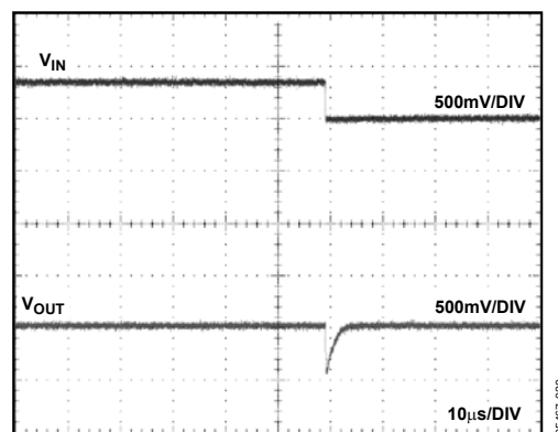
Figure 24. ADR361 Line Transient Response (Decreasing), No Capacitors
