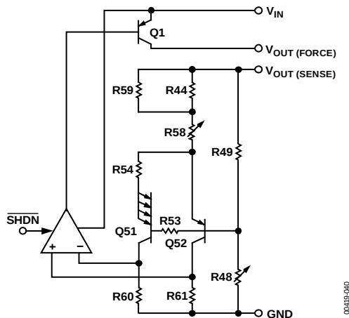
Figure 33. Simplified Schematic
