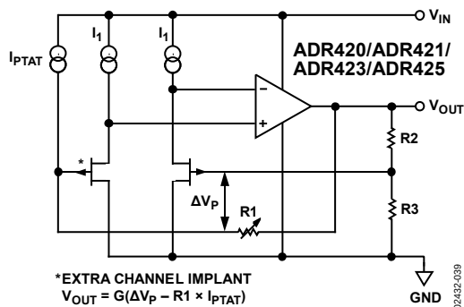
Figure 38. Simplified Schematic
