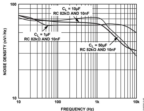
Figure 33. Noise with Compensation Network
