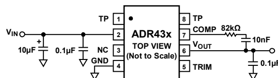
Figure 32. Compensated Reference
