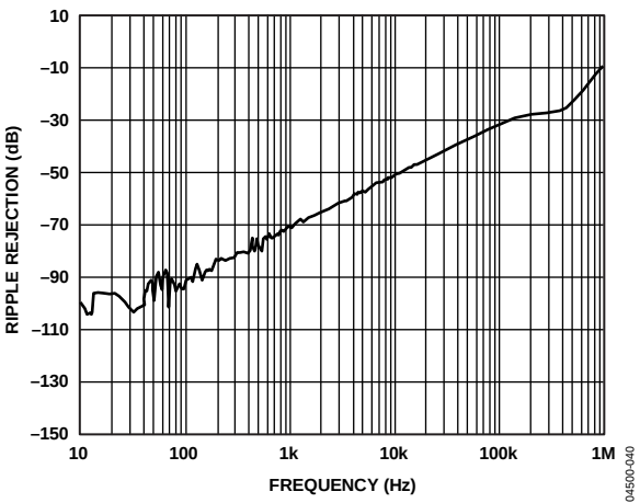
Figure 28. Ripple Rejection
