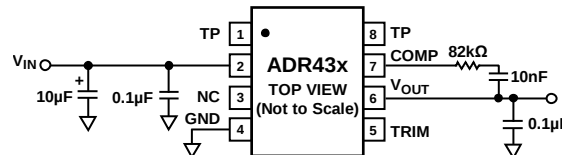
Figure 32. Compensated Reference
