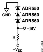
Figure 23. -15 V Output with Stacked ADR550s
