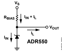
Figure 19. Shunt Reference
