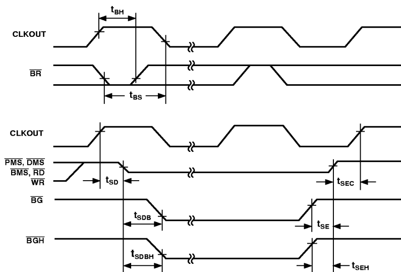
Figure 10. Bus Request–Bus Grant
