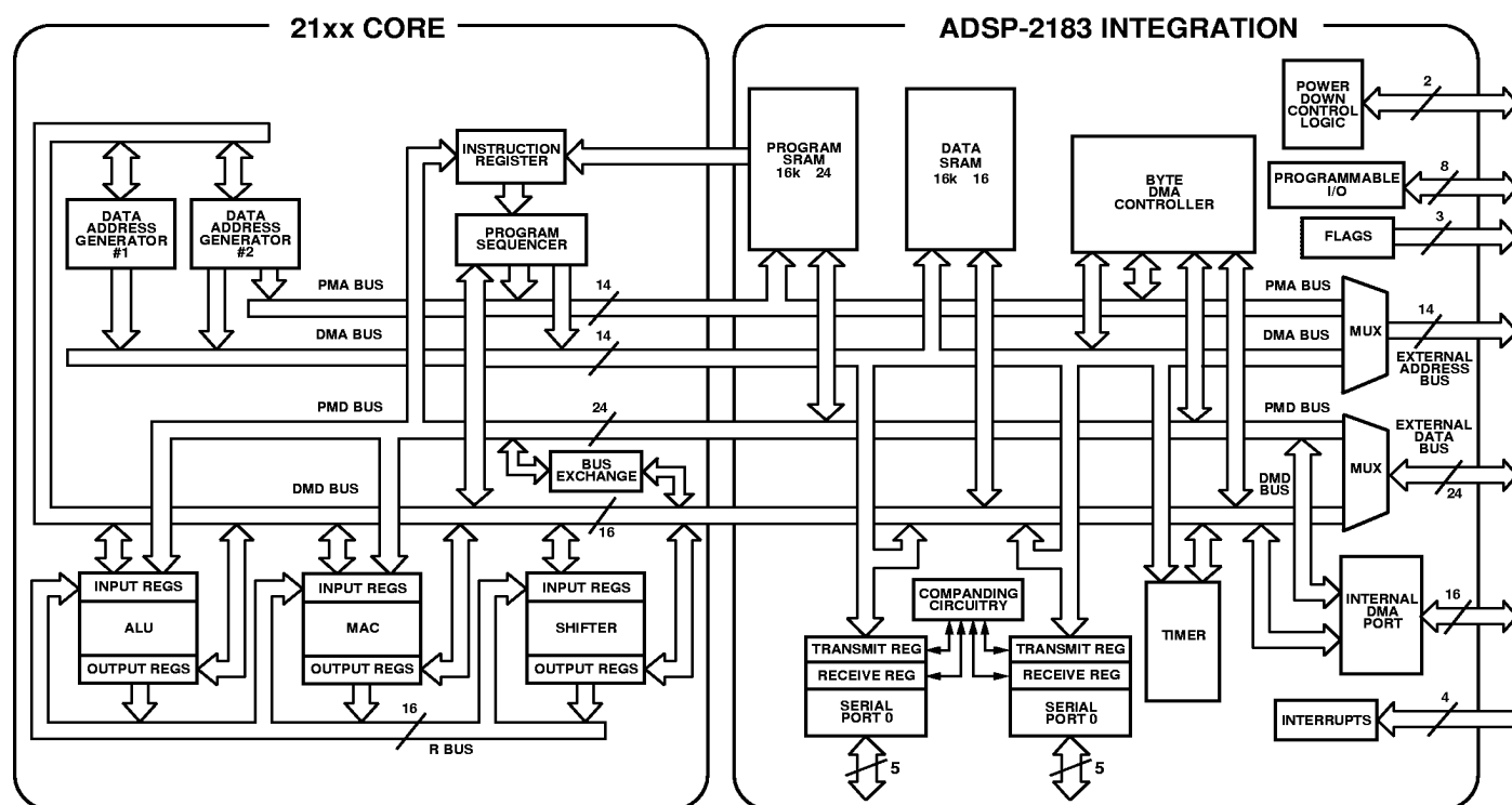
Figure 1. Block Diagram
