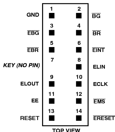
Figure 7. Target Board Connector for EZ-ICE
