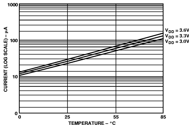
Figure 19. Typical Drive Currents
