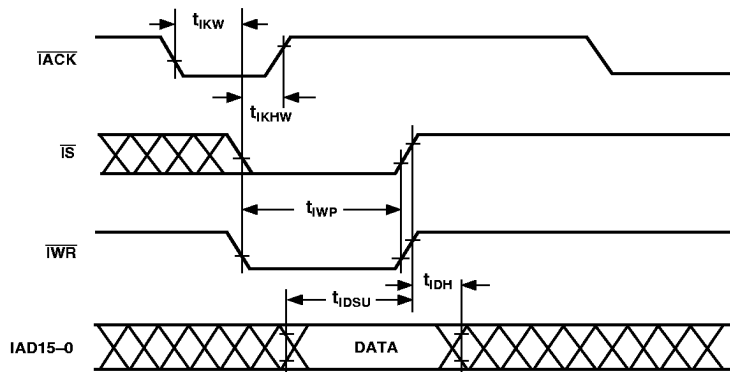
Figure 15. IDMA Write, Short Write Cycle
