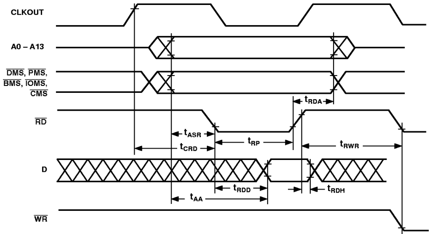
Figure 11. Memory Read
