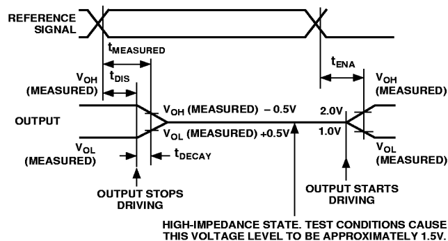
Figure 25. Output Enable/Disable
