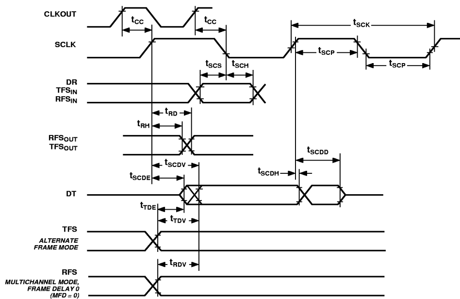
Figure 13. Serial Ports
