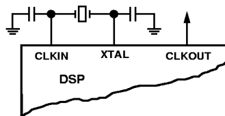
Figure 3. External Crystal Connections
