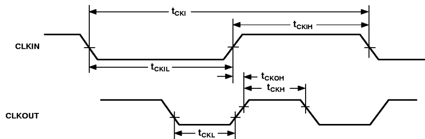
Figure 8. Clock Signals
