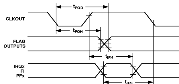
Figure 9. Interrupts and Flags
