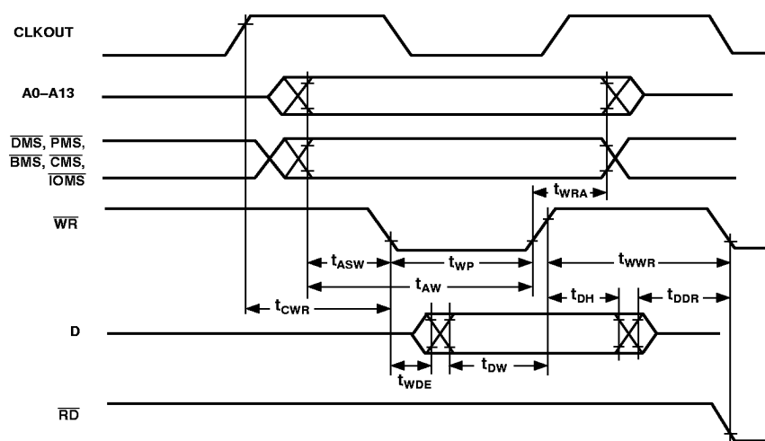
Figure 12. Memory Write
