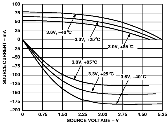
Figure 19. Typical Drive Currents
