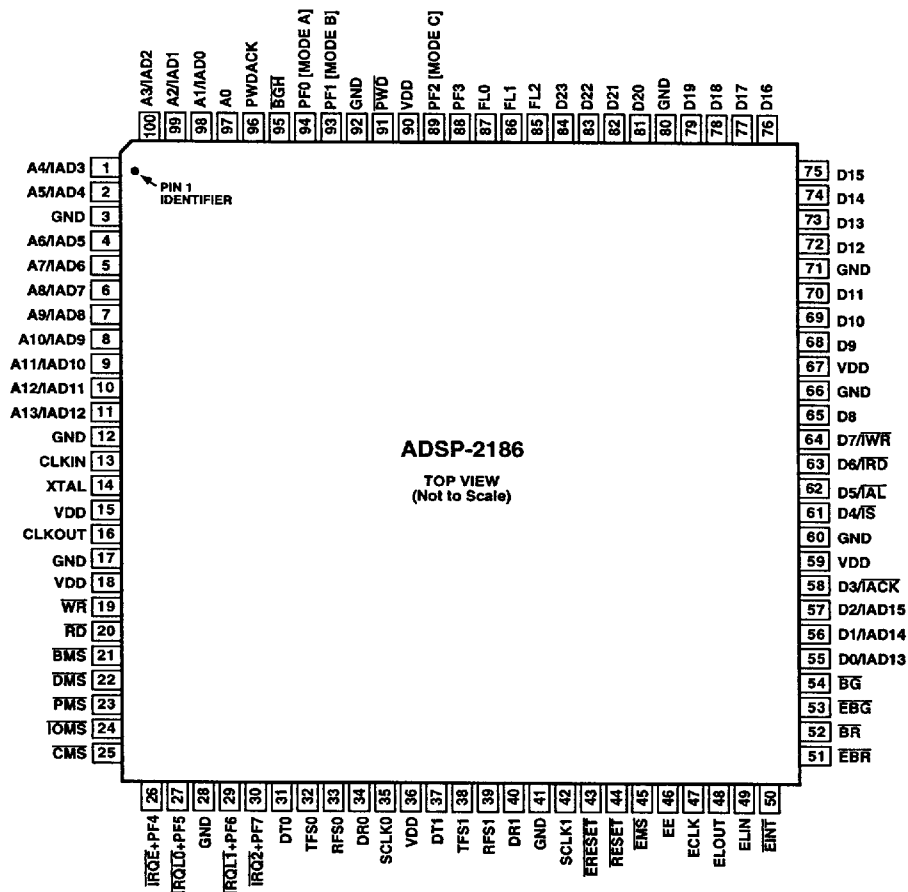
100-Lead TQFP Package Pinout
