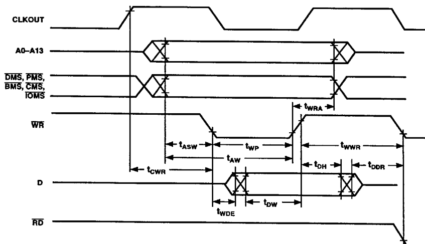
Figure 18. Memory Write
