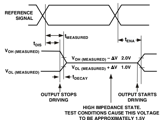
Figure 18. Output Enable/Disable
