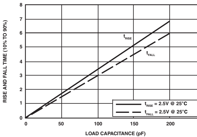
Figure 61. Driver Type A Typical Rise and Fall Times (10%–90%) vs. Load Capacitance ( 2.5V V_{DDEXT}/V_{DDMEM} )
