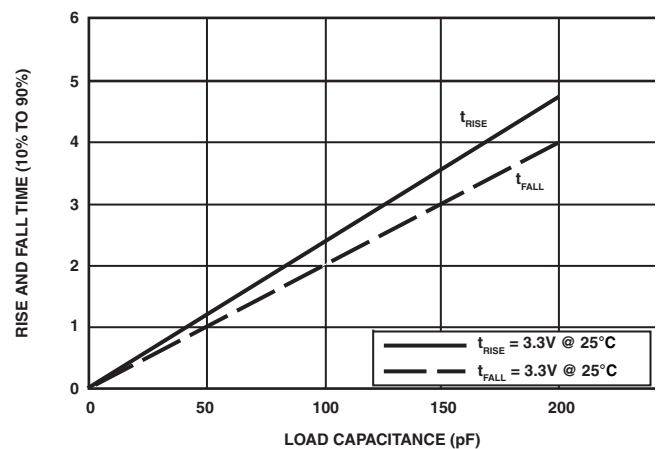
Figure 65. Driver Type B Typical Rise and Fall Times (10%–90%) vs. Load Capacitance ( 3.3V V_{DDEXT}/V_{DDMEM} )
