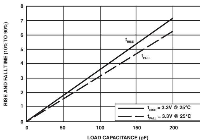
Figure 71. Driver Type D Typical Rise and Fall Times (10%–90%) vs. Load Capacitance ( 3.3V_{DDEXT}/V_{DDMEM} )
