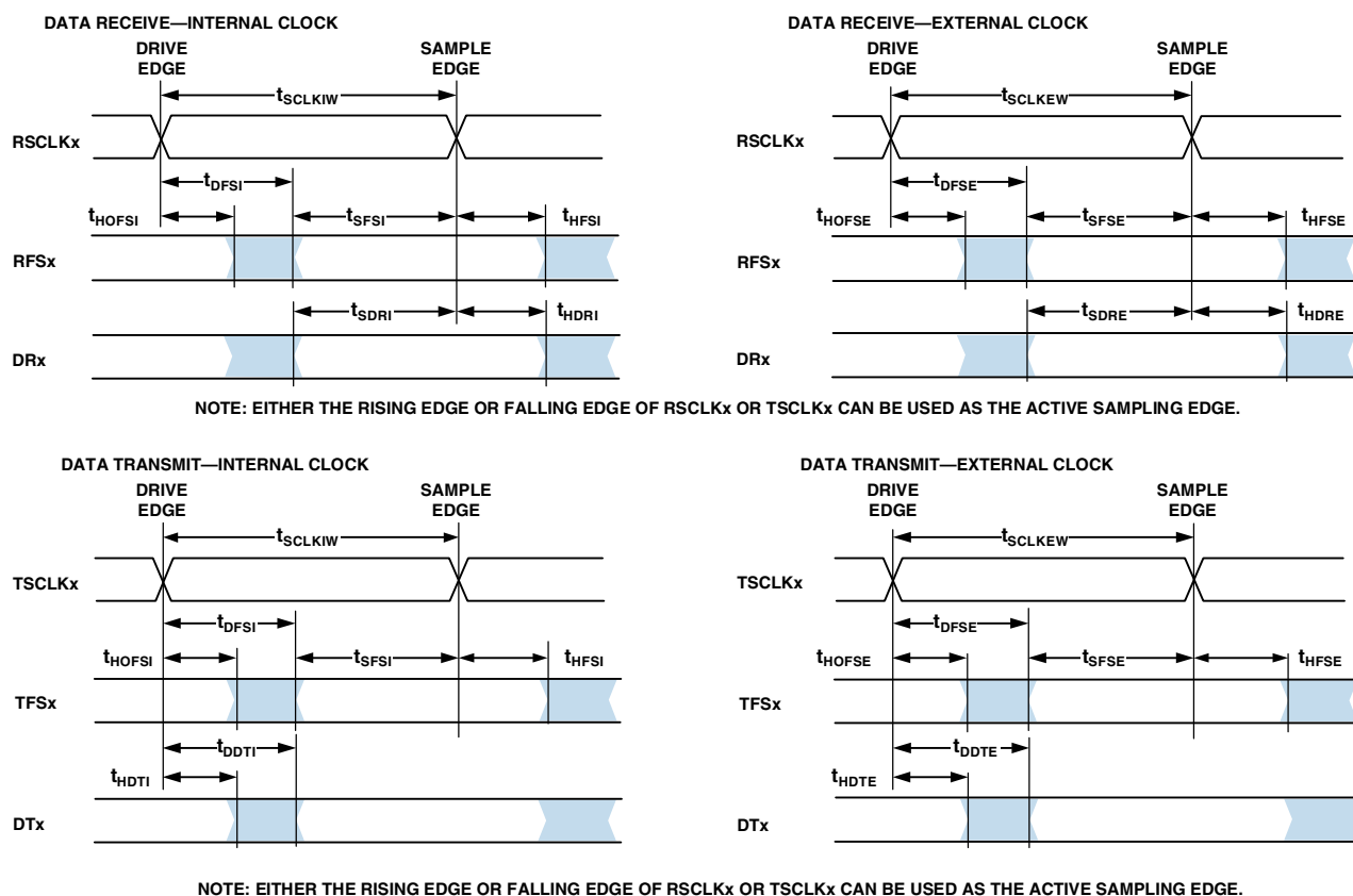
Figure 23. Serial Ports
