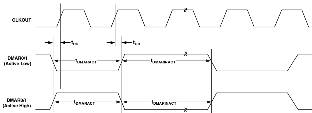
Figure 18. External DMA Request Timing
