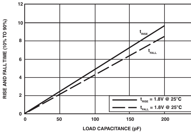
Figure 60. Driver Type A Typical Rise and Fall Times (10%–90%) vs. Load Capacitance ( 1.8V V_{DDEXT}/V_{DDMEM} )
