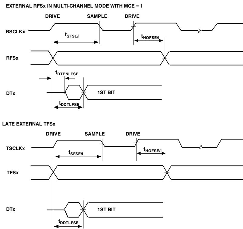
Figure 25. Serial Ports — External Late Frame Sync
