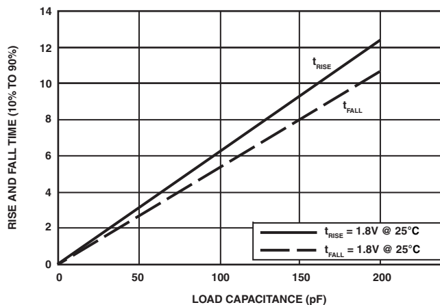
Figure 69. Driver Type D Typical Rise and Fall Times (10%–90%) vs. Load Capacitance ( 1.8V_{DDEXT}/V_{DDMEM} )
