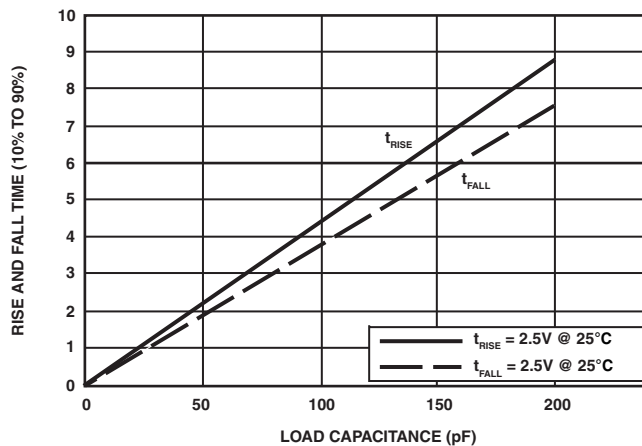
Figure 70. Driver Type D Typical Rise and Fall Times (10%–90%) vs. Load Capacitance ( 2.5V_{DDEXT}/V_{DDMEM} )
