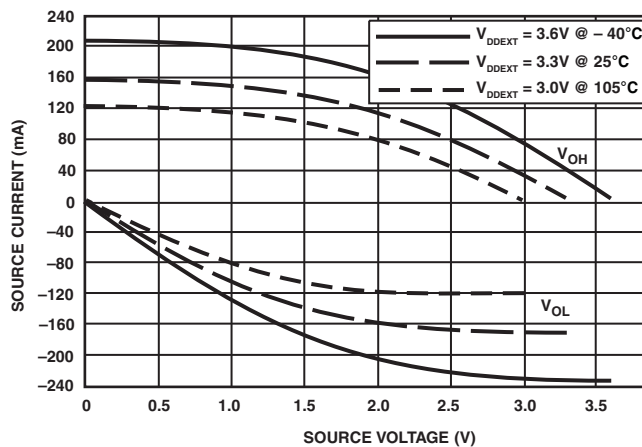
Figure 45. Driver Type B Current ( 3.3V V_{DDEXT}/V_{DDME} )
