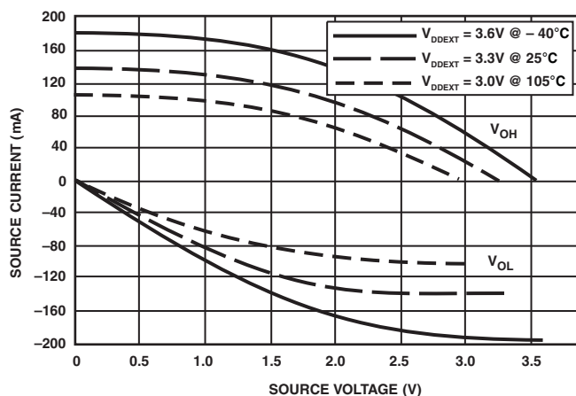
Figure 42. Driver Type A Current ( 3.3V V_{DDEXT}/V_{DDME} )
