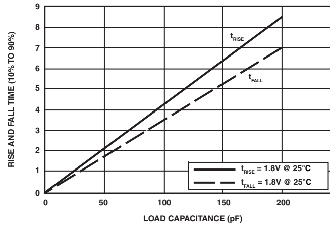
Figure 63. Driver Type B Typical Rise and Fall Times (10%–90%) vs. Load Capacitance ( 1.8V V_{DDEXT}/V_{DDMEM} )
