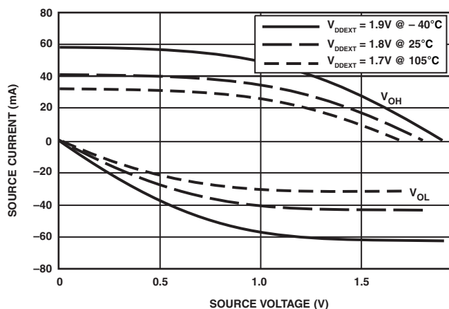
Figure 44. Driver Type A Current ( 1.8V V_{DDEXT}/V_{DDME} )
