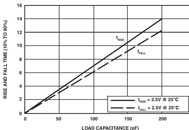
Figure 67. Driver Type C Typical Rise and Fall Times (10%–90%) vs. Load Capacitance ( 2.5V_{DDEXT}/V_{DDMEM} )
