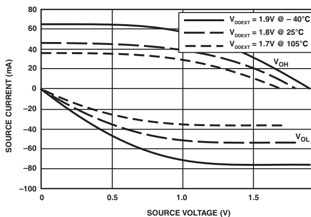
Figure 47. Driver Type B Current ( 1.8V V_{DDEXT}/V_{DDME} )
