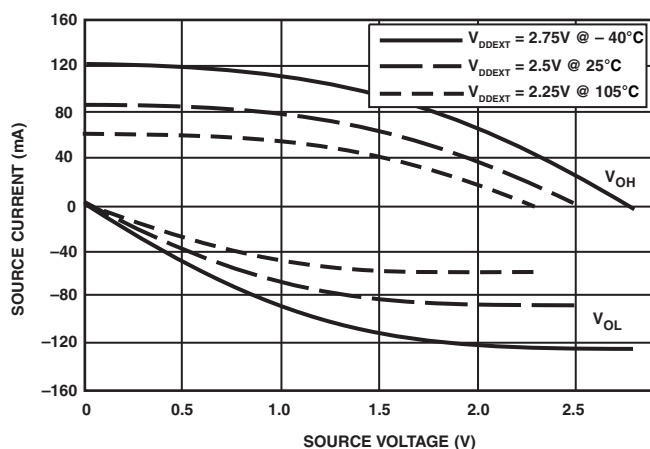
Figure 43. Driver Type A Current ( 2.5V V_{DDEXT}/V_{DDME} )
