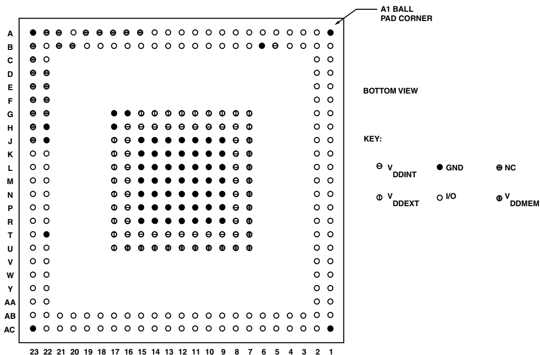
Figure 73. 289-Ball CSP_BGA Ball Configuration (Bottom View)
