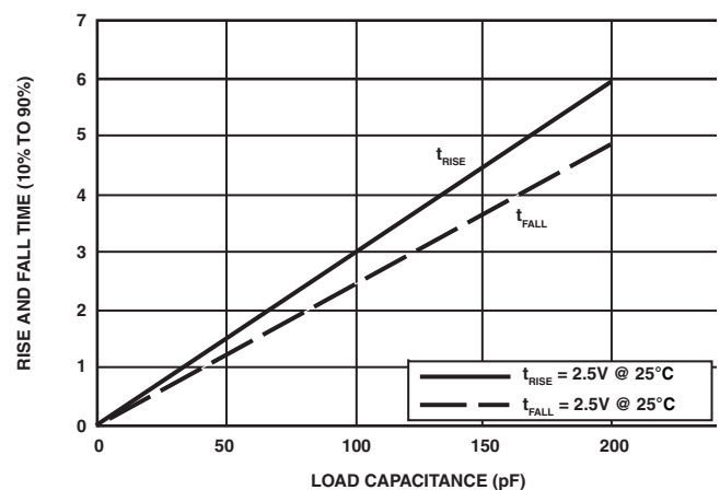
Figure 64. Driver Type B Typical Rise and Fall Times (10%–90%) vs. Load Capacitance ( 2.5V V_{DDEXT}/V_{DDMEM} )
