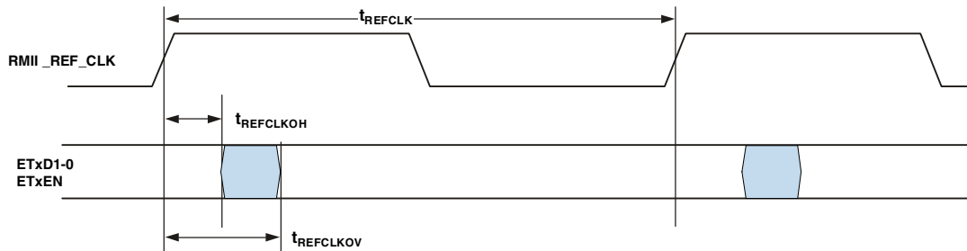
Figure 38. 10/100 Ethernet MAC Controller Timing: RII Transmit Signal
