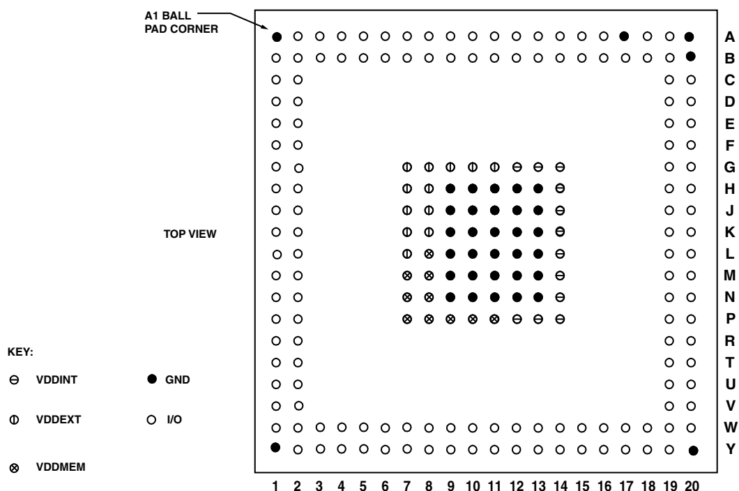
Figure 74. 208-Ball CSP_BGA Ball Configuration (Top View)
