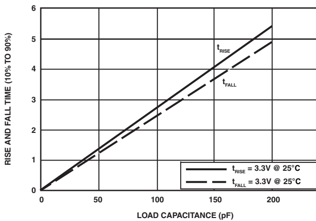
Figure 62. Driver Type A Typical Rise and Fall Times (10%–90%) vs. Load Capacitance ( 3.3V V_{DDEXT}/V_{DDMEM} )
