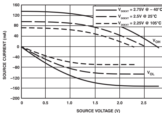
Figure 46. Driver Type B Current ( 2.5V V_{DDEXT}/V_{DDME} )
