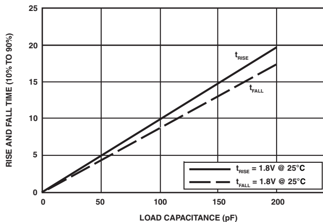
Figure 66. Driver Type C Typical Rise and Fall Times (10%–90%) vs. Load Capacitance ( 1.8V_{DDEXT}/V_{DDMEM} )
