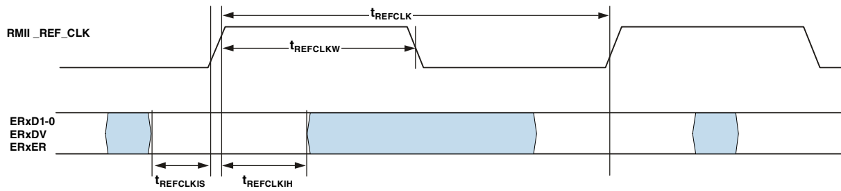
Figure 37. 10/100 Ethernet MAC Controller Timing: RII Receive Signal
