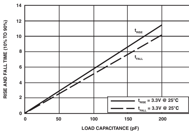
Figure 68. Driver Type C Typical Rise and Fall Times (10%–90%) vs. Load Capacitance ( 3.3V_{DDEXT}/V_{DDMEM} )
