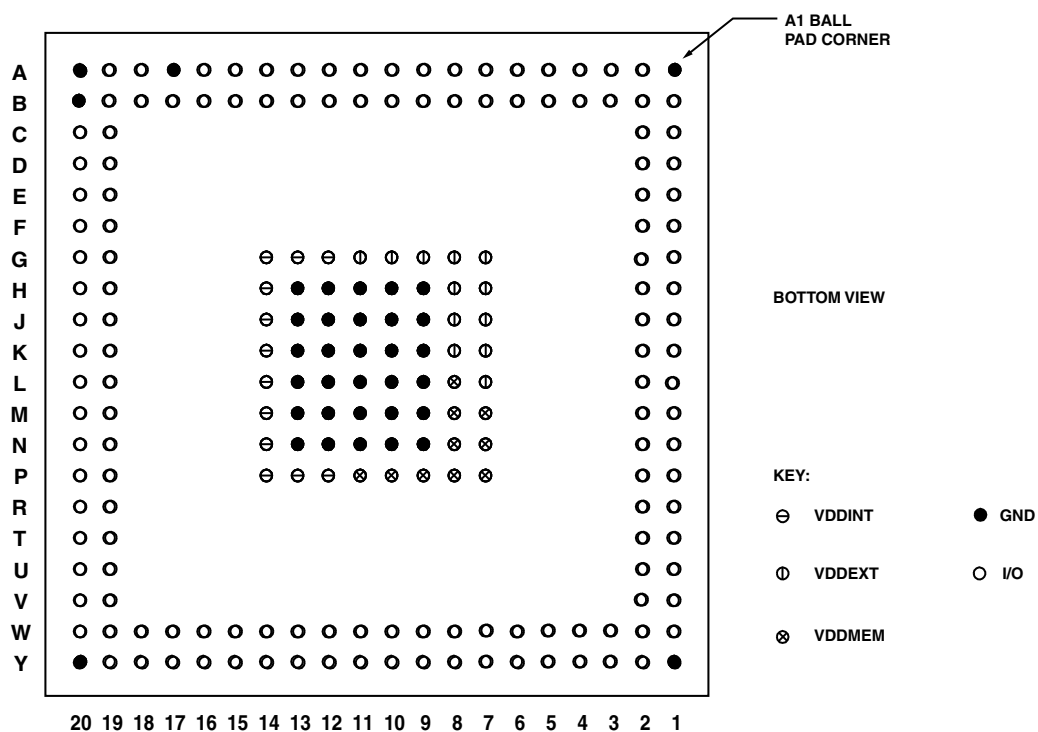
Figure 75. 208-Ball CSP_BGA Ball Configuration (Bottom View)
