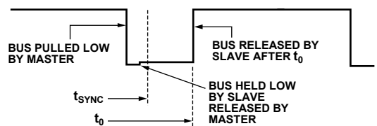
Figure 55. BSD Slave Transmitting 0
