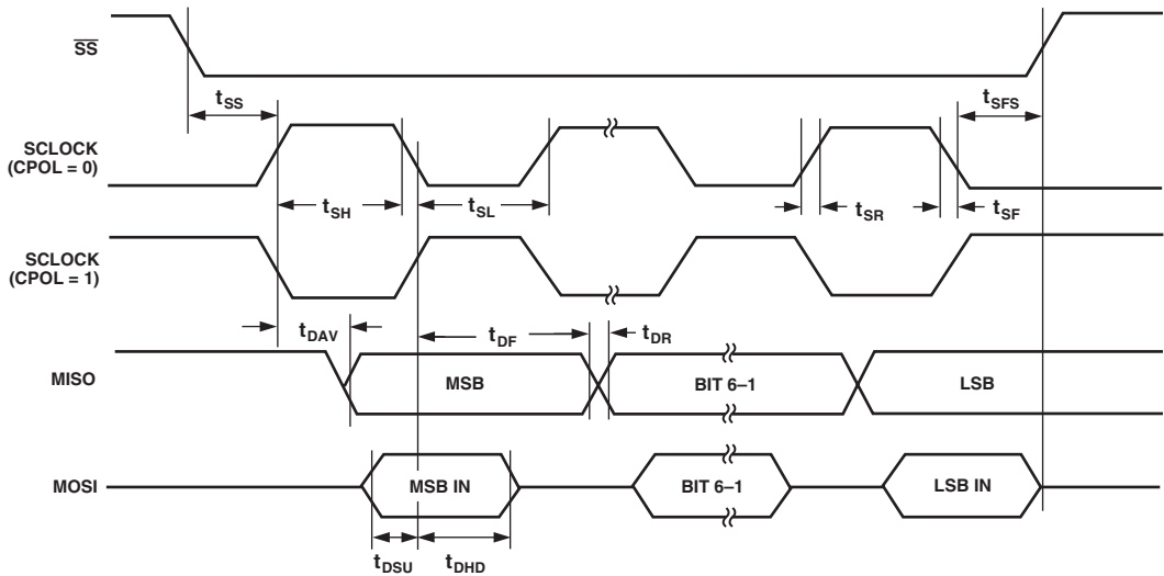
Figure 58. SPI Slave Mode Timing (CPHA = 1)
