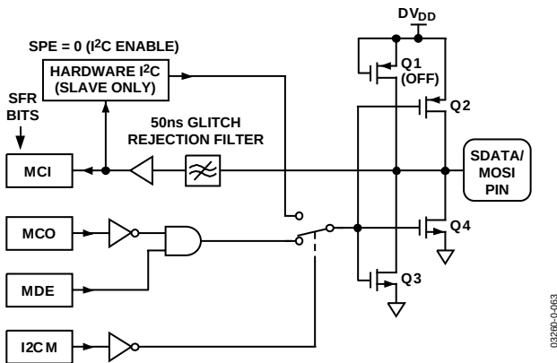
Figure 65. SDATA/MOSI Pin I/O Functional Equivalent in I 2 C Mode
