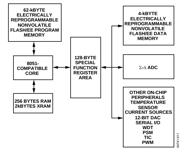
Figure 11. Programming Model
