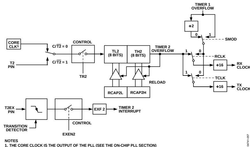
Figure 60. Timer 2, UART Baud Rates
