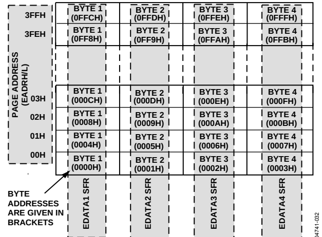
Figure 32. Flash/EE Data Memory Control and Configuration
