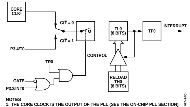
Figure 54. Timer/Counter 0, Mode 2
