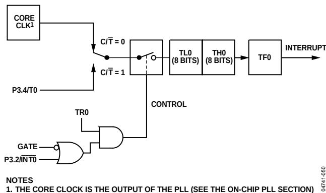
Figure 53. Timer/Counter 0, Mode 1
