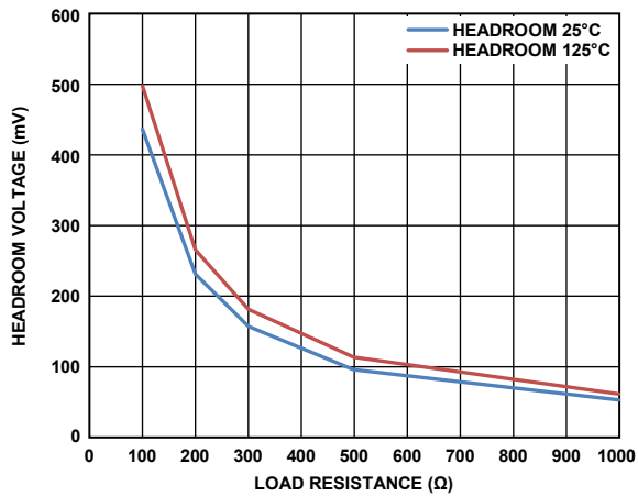
Figure 8. Typical Headroom Voltage vs. Load Resistance for VDACC7, VDACV_{DD} = 3\text{ V} ; Headroom = VDACV_{DD} - VDAC\text{ Output Voltage}
