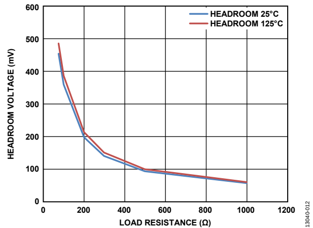
Figure 12. Typical Headroom Voltage vs. Load Resistance for VDACC4, AV_{DD} = 3\text{ V} ; Headroom = AV_{DD} - VDAC\text{ Output Voltage}
