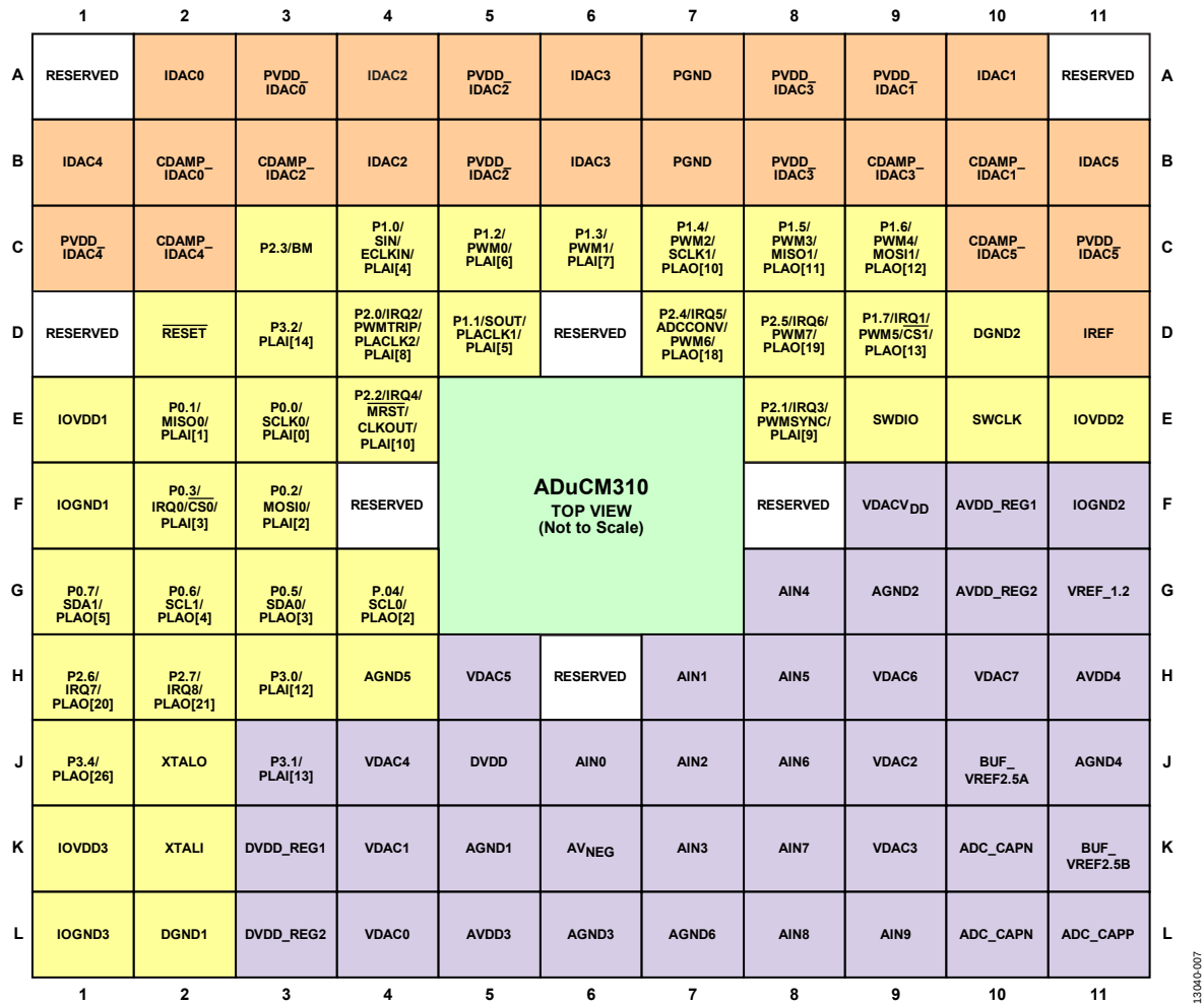
Figure 7. Pin Configuration
