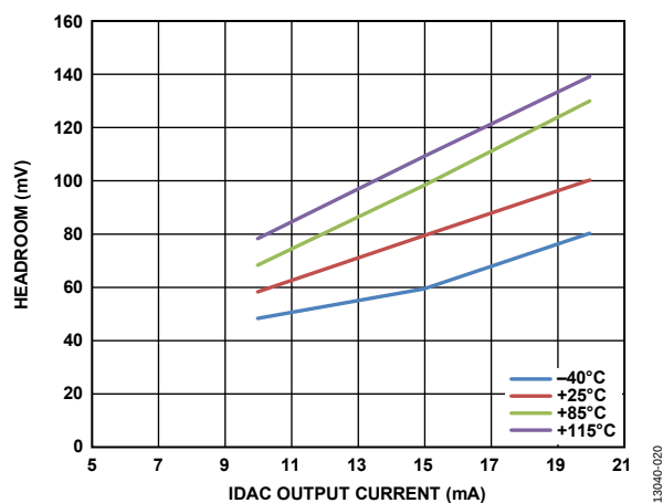
Figure 20. Typical IDAC5 PVDD_IDAC5 Pin Voltage Headroom vs. Output Current for Different Temperatures, PV_{DD} = 1.8\text{ V}
