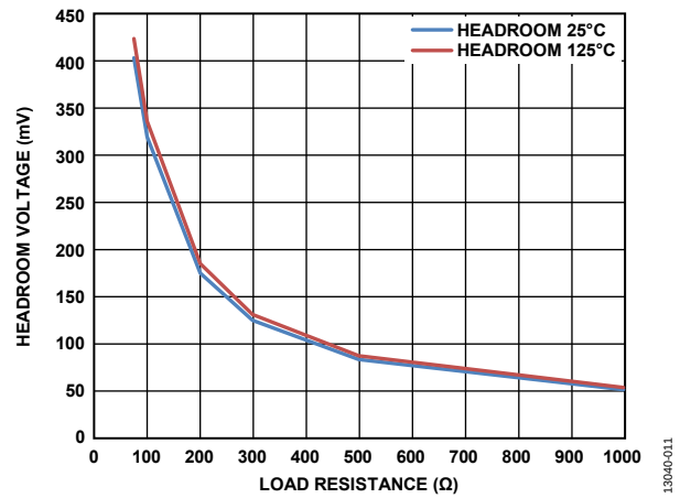
Figure 11. Typical Headroom Voltage vs. Load Resistance for VDACC0, AV_{DD} = 3\text{ V} ; Headroom = AV_{DD} - VDAC\text{ Output Voltage}
