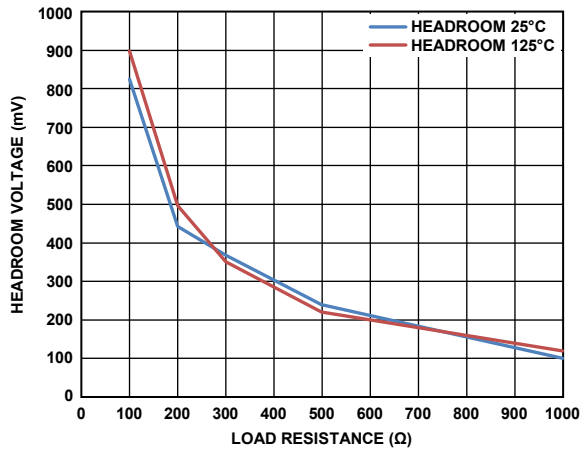
Figure 10. Typical Headroom Voltage vs. Load Resistance for VDACC2, AV_{NEG} = -5\text{ V} ; Headroom = AV_{NEG} - VDAC\text{ Output Voltage}
