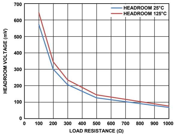
Figure 9. Typical Headroom Voltage vs. Load Resistance for VDACC7, VDACV_{DD} = 5\text{ V} ; Headroom = VDACV_{DD} - VDAC\text{ Output Voltage}
