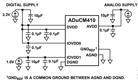
Figure 16. External Multiple Supply Connections
