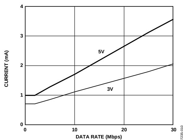
Figure 10. Typical ADuM2200 V_{DD2} Supply Current vs. Data Rate for 5 V and 3 V Operation
