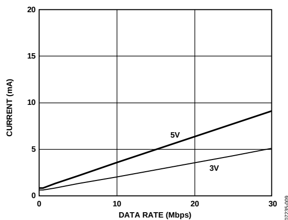
Figure 9. Typical ADuM2200 V_{DD1} Supply Current vs. Data Rate for 5 V and 3 V Operation
