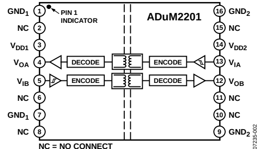
Figure 2. ADuM2201
