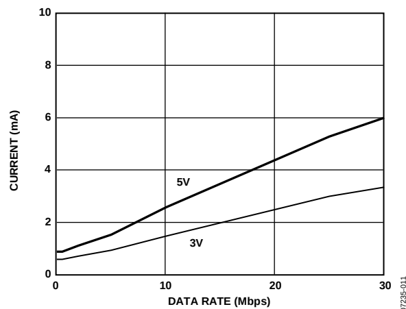
Figure 11. Typical ADuM2201 V_{DD1} or V_{DD2} Supply Current vs. Data Rate for 5 V and 3 V Operation
