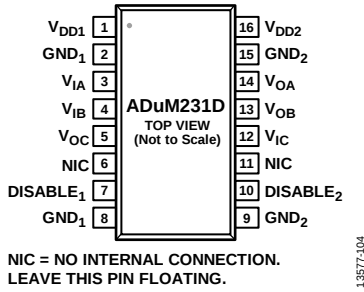
Figure 8. ADuM231D Pin Configuration
