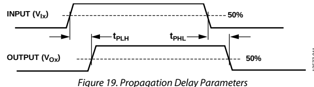
Figure 19. Propagation Delay Parameters
