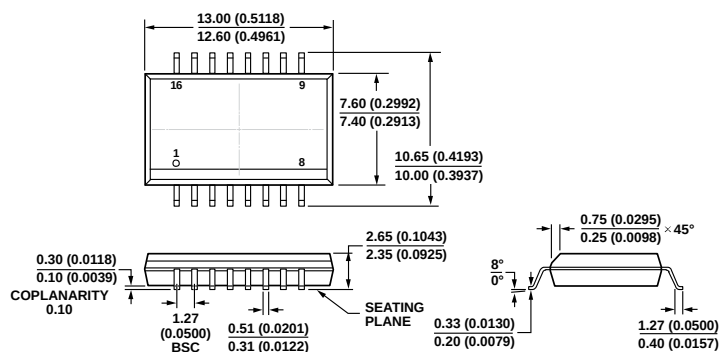
Figure 24. 16-Lead Standard Small Outline Package [SOIC_W] Wide Body (RW-16)
